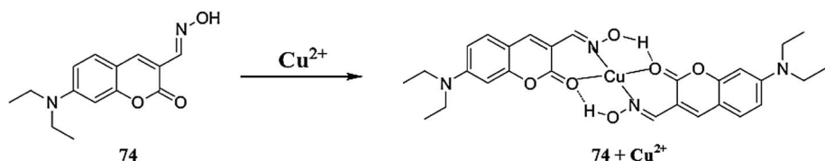
Fig. 65 Chemical structure of receptor 74 and the proposed copper complexation mechanism.
