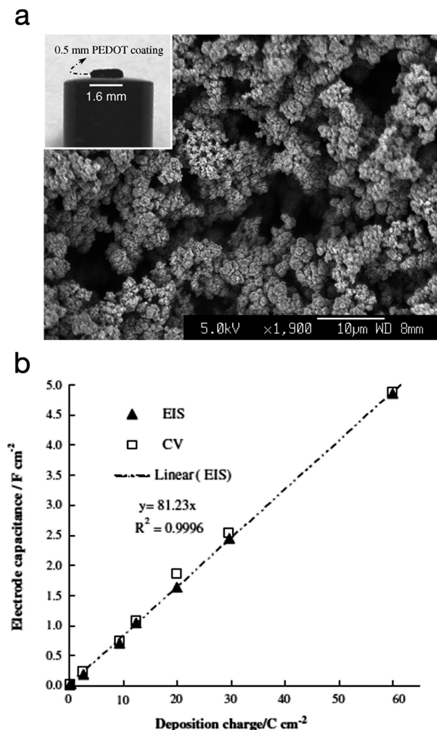
Fig. 18 (a) SEM micrograph of PEDOT electropolymerised via potentiostatic polymerisation (deposition charge: 30 \text{ C cm}^{-2} ). Inset: photograph of a PEDOT film ( 60 \text{ C cm}^{-2} ) on a Pt disc electrode. (b) Plot of the electrode specific capacitance as a function of polymerisation charge. Values measured by electrochemical impedance spectroscopy (EIS) and cyclic voltammetry (CV) are both presented. Reprinted from ref. 89 with permission from Elsevier.
