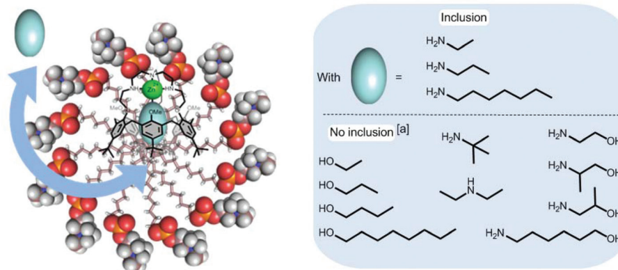
Fig. 3 Summary, using a schematic representation, of the host–guest properties of the receptor 1\cdot\text{Zn}^{2+} incorporated in DPC micelles. [a]: see ESI† for experimental conditions. 21
