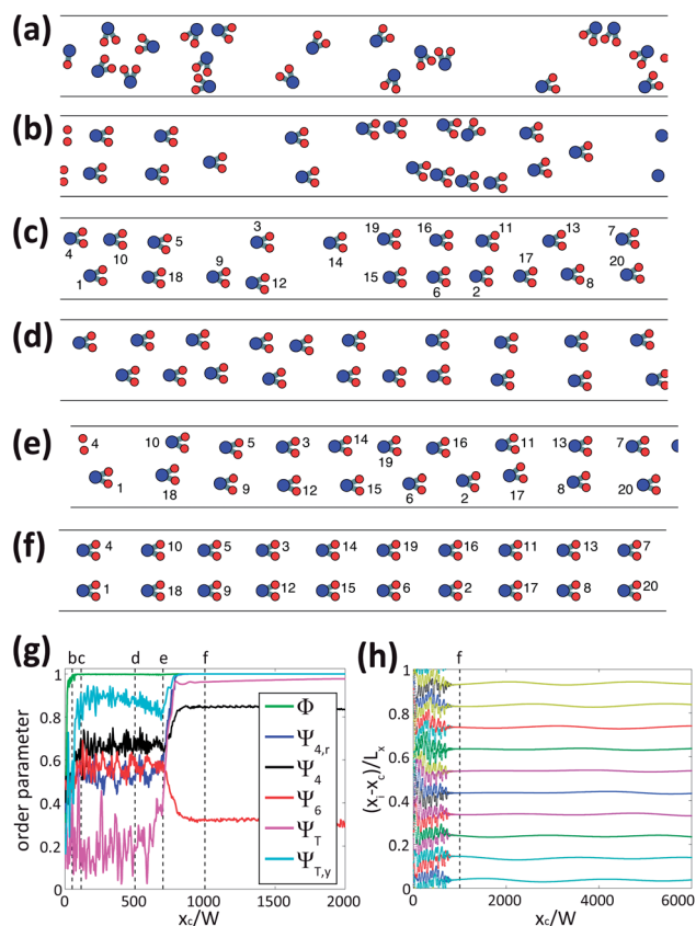
Fig. 7 A suspension of trumbells can self-organize into a two-dimensional crystal. There are N = 20 particles with \tilde{W} = 20 and L_x/W = 7.5 . (a) Trumbells are initially placed with random positions and angles. (b) The particles have aligned with the flow. Groups of particles have locally self-organized, either laterally, as doublets, or in the streamwise direction, as strings held together by the quadrupolar interaction. (c) The particles have entirely partitioned into two separate lanes located near the doublet positions y = W/4 and y = 3W/4 . In this case, the two lanes have an equal number of particles. However, not every particle has found a partner. For some particles the partner position is vacant (e.g. particle 9.) For others, the partner is shared (e.g. particles 4, 10, 1) in a triangular configuration. (d) The particles have spread more evenly across the channel, but vacancies and triangle formations remain. (e) The suspension now resembles a strained crystal, and is on the threshold of relaxation to an unstrained lattice. Particle 2 will capture particle 16, allowing 6 and 19 to partner. (f) The particles have settled into an apparently “perfect” crystal, and have approximately the same neighbors as in frame (c). (g) Evolution of the order parameters with center of mass position x_c . Dashed lines correspond to the frames shown previously. (h) Long time evolution of the particle positions in the streamwise direction. Aside from a small amplitude, low frequency density wave, particles positions in x are approximately evenly spaced and steady.
