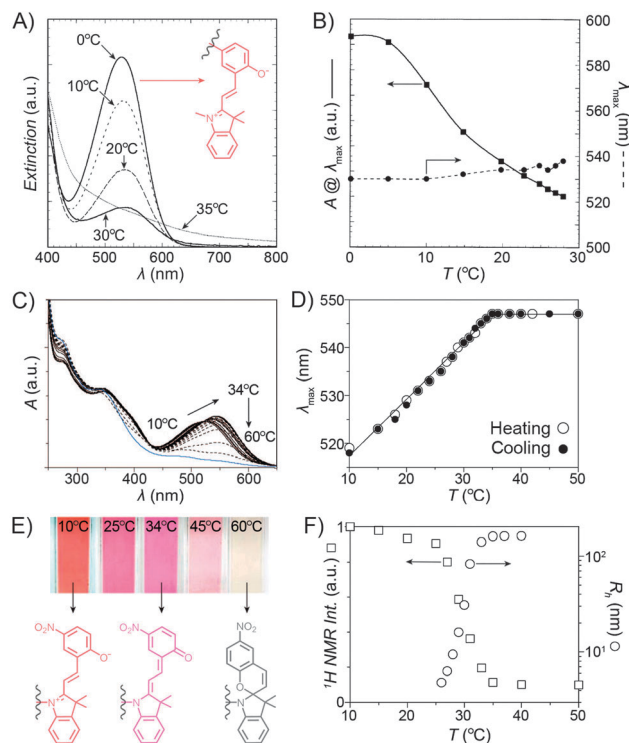
Fig. 9 Spiropyran as a probe for microenvironment polarity. (A) Thermally induced MC \rightarrow SP transition (0–30 ^\circ\text{C} ) precedes precipitation of poly(NIPAM-SP) (35 ^\circ\text{C} ). (B) Changes in maximum absorbance values and wavelength absorption maxima at temperatures below the volume phase transition. (C) Optical response of a poly(NIPAM-SP) polymer pre-irradiated with UV as it is gradually heated from T = 10^\circ\text{C} to T = 60^\circ\text{C} . (D) Temperature-dependent changes in wavelength absorption maxima of the same copolymer. (E) Colour changes accompanying a gradual zwitterion \rightarrow quinoid conversion (observed spectrophotometrically in (C)). (F) Precipitous drop of the integrated intensity of the NIPAM's CH proton resonances (left) coincides with the rapid increase of the hydrodynamic radius (right). [Adapted with permission from ref. 223 (Copyright 2004 American Chemical Society) (A and B) and ref. 224 (Copyright 2009 American Chemical Society) (C–F).]
