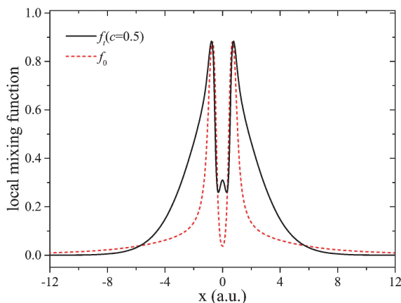
Fig. 8 Comparison of f_0(\mathbf{r}) and f_1(\mathbf{r}) with c = 0.5 for the C atom along the x -axis.
