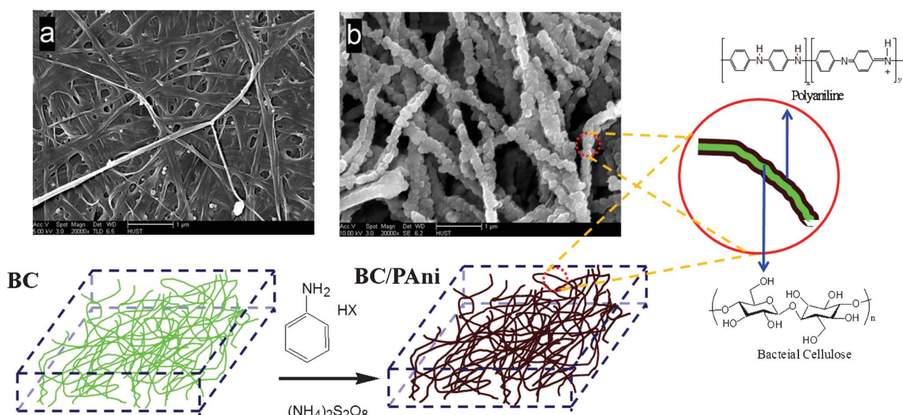
Fig. 4 Schematic diagram of the process of aniline polymerization in the BC hydrogel. (Fig. a is the FESEM image of the hot-pressed BC membrane; and Fig. b is the FESEM image of hot-pressed BC-PAni membrane.)
