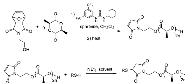
Scheme 23 The synthesis of \alpha -functional thioether polyactides via ring-opening polymerization of lactide with a furan-protected maleimide initiator followed by a [4 + 2] cycloreversion and base-mediated thiol-ene coupling.
