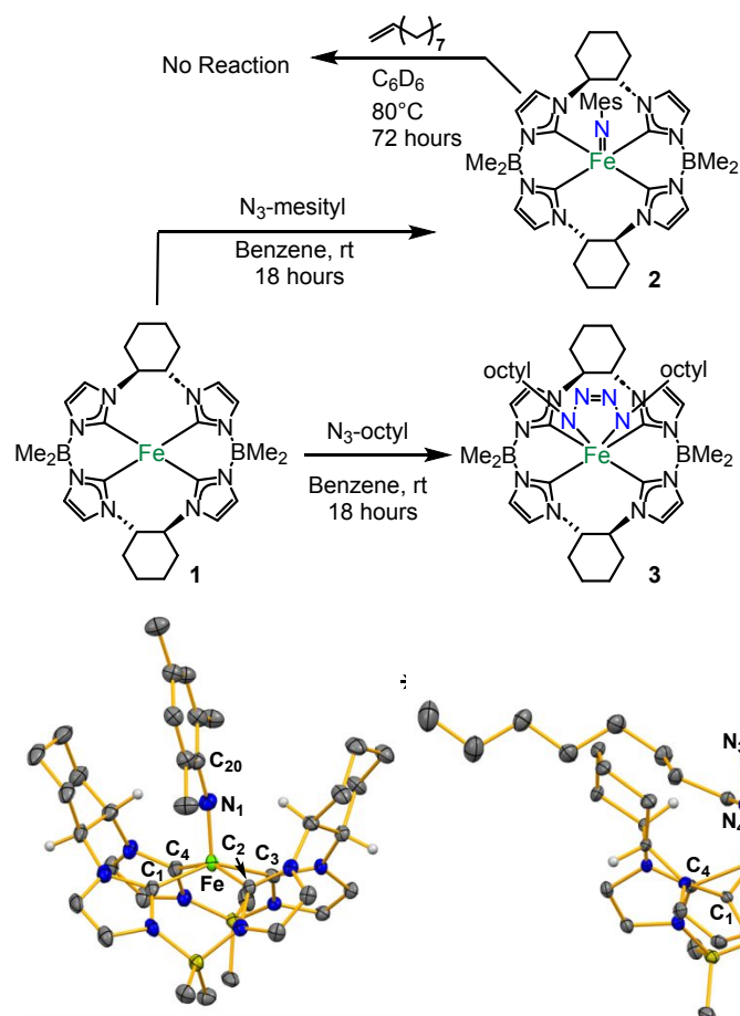
Scheme 1. Reactions of 1 with both aryl and alkyl azides.
