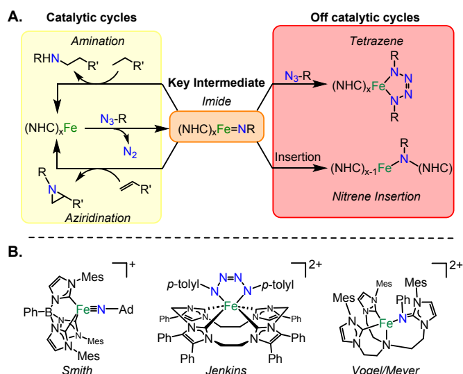
Fig. 1. (A) Possible reactivities of (\text{NHC})_x\text{Fe} complexes with organic azides. Notably, additional off-cycle reactions can occur from a metal imide. (B) Examples of the first imide, tetrazene, and imide insertion supported by NHC auxiliary ligands that were formed from organic azides.
