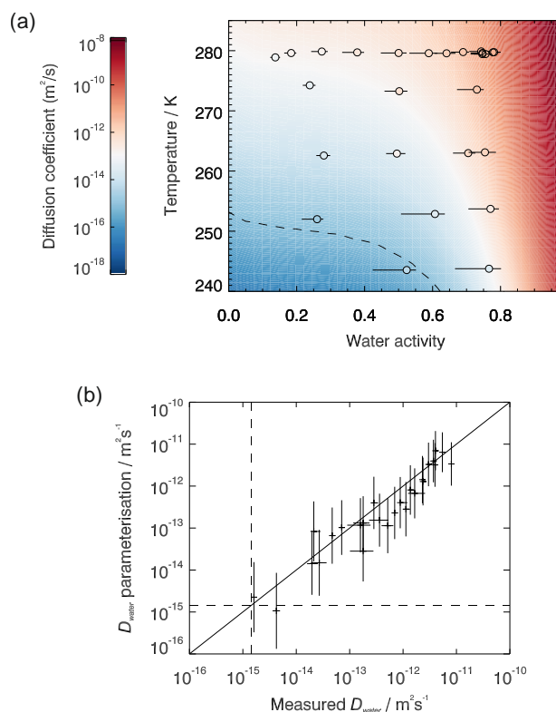
Fig. 1. (a) Diffusion coefficients of water in SOM. Experimental data points are shown as coloured circles and the fit is the shaded background, both coloured on the same scale. The differences in colour between the background and circle interiors show the difference between the fit and the measured data points. Multiple measurements were performed at a water activity of 0.75 and 280 K over the course of 4 months to verify that the diffusive properties of the sample did not change with age. These datapoints are shown to be in good agreement with each other and the fit. (b) A one-to-one plot showing the measured water diffusion coefficients vs the parameterisation. The dashed lines mark the regions above which the half-time for water diffusion into a spherical droplet of radius 100 nm is less than 1 s.
