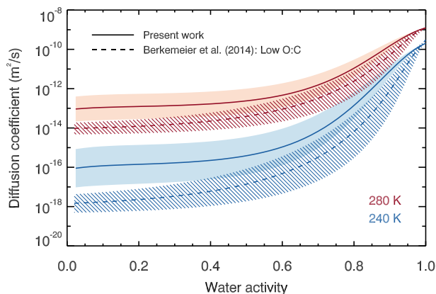
Fig. 3. The fit to our experimental data (solid lines and shaded error regions) compared with the semi-empirical low oxidation predictions from Berkemeier, et al. 53 (dotted lines and hatched error regions) at 280 K and 240 K.
