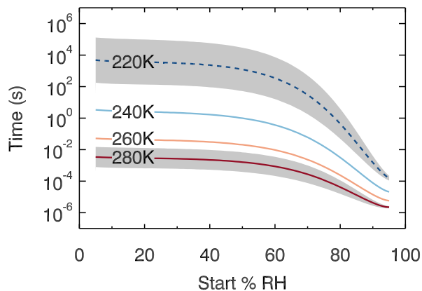
Fig. 5. Modelled times for an increase in water activity of 0.01 at the centre of a 100 nm diameter particle following a 2% step up in RH. Below 240 K we use an extrapolation of our water diffusion coefficient fit, indicated by a dotted line. Timescales for equivalent steps down in RH are very similar. The grey shaded region indicates our estimated uncertainty (see Supplementary Information for details of error analysis).
