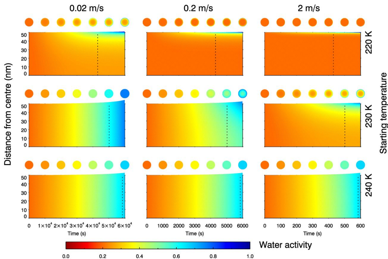
Fig. 6. Water activity across droplet radius as a 100 nm particle follows an updraft of 0.02, 0.2 and 2 m/s (left to right) with temperature decreasing according to the dry adiabatic lapse rate and fixed water vapour partial pressure. Droplets start in equilibrium with their surrounding RH at a homogeneous water activity of 0.2, at a temperature of 220, 230 or 240 K (top to bottom). The resulting changes in RH and temperature with time are shown in Supplementary Fig. 7. The dotted lines indicate the point at which the RH_{ice} increases above 100% and heterogeneous nucleation is feasible.
