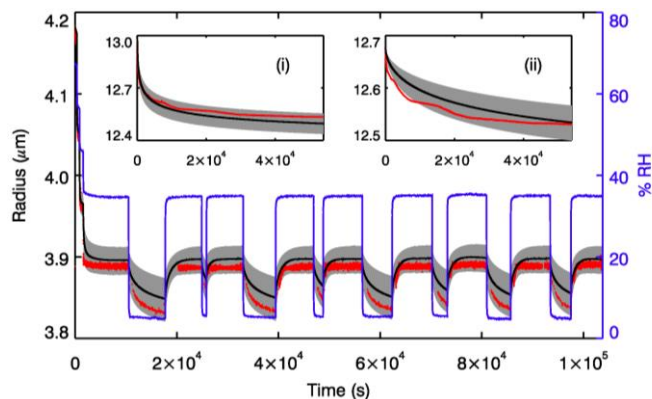
Fig. 4. The main plot shows the changing radius of a sucrose droplet following a repeatedly stepped RH profile (blue line) at room temperature, measured using optical tweezers (red points). The same RH profile was run through the model for a droplet with 1000 shells; the output radius is shown by the black line, with the grey shaded region corresponding to the error in the measured RH of \pm 2\% . Inset (i) shows the size change recorded in an EDB for a 13.03 \mu\text{m} droplet confined and equilibrated at 53% RH experiencing a rapid step change (half-time for RH change < 1 s) to 20% RH (red line). The equivalent model output is shown in black, run with 3000 shells, with the grey region corresponding to a \pm 2\% error in starting water activity and chamber RH. Similarly, inset (ii) shows the size change recorded in an EDB for a 12.68 \mu\text{m} droplet confined and equilibrated at 35% RH experiencing a rapid step change to 15% RH (red line). Again, the model output is shown in black, with the grey region corresponding to a \pm 2\% error in starting water activity and chamber RH. Uncertainties in the experimentally determined radii are estimated to be \pm 50 nm.
