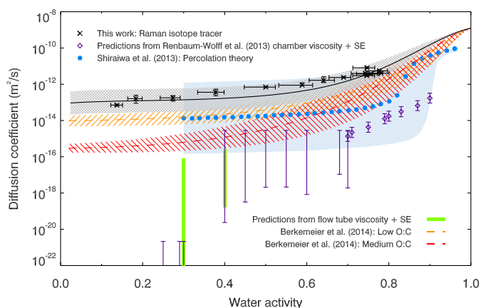
Fig. 2. Comparison of measured diffusion coefficients of water in \alpha -pinene SOM with literature data. Laboratory measurements at 280 K (black crosses, with our parameterisation shown as a black line, with grey shaded uncertainty region) are compared with predictions from percolation theory at room temperature (blue circles, with blue shaded uncertainty region 30 ) and the semi-empirical method used by Berkemeier, et al. 53 for low (orange dashed line and hatched error region, O:C = 0.3) and medium (red dashed line and hatched error region, O:C = 0.5) oxidation states at 280 K. Also shown are the diffusion coefficients predicted by the Stokes-Einstein (S-E) equation with a hydrodynamic diameter of water of 2 Å, using the room temperature viscosity measurements on chamber-generated \alpha -pinene SOM by Renbaum-Wolff, et al. 11 (generated using 80-100 ppb \alpha -pinene and 300 ppb ozone, purple diamonds and bars), and on flow tube-generated \alpha -pinene SOM (generated using 5 ppm \alpha -pinene and 12 ppm ozone, green bars).
