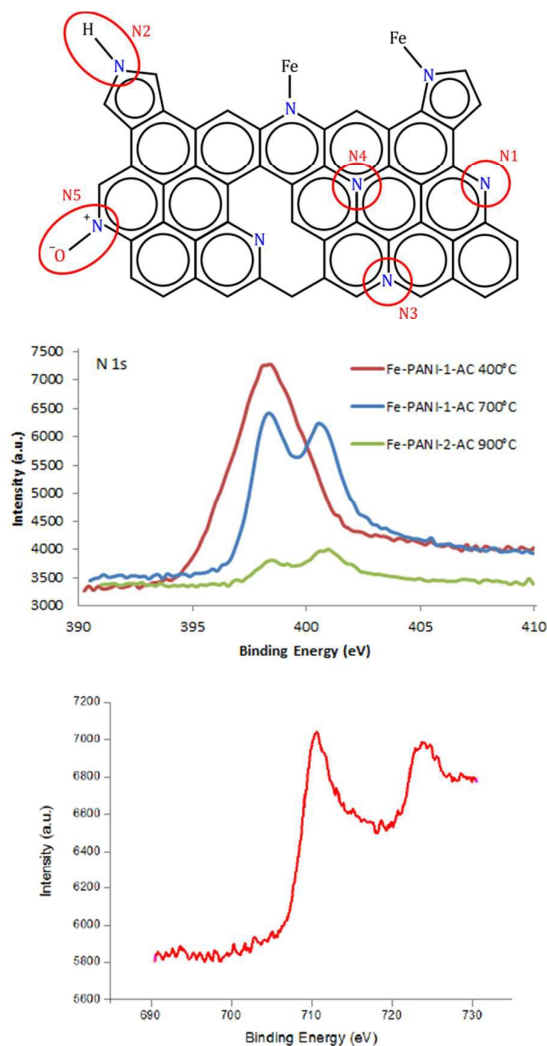
Figure 4. Top: Representation of a graphitic carbon material with the different possible N configurations. Middle: N1s XPS signal as a function of the pyrolysis temperature used in the synthesis of Fe-PANI-AC. Bottom: Fe 2p XPS signal of Fe-PANI-AC-1.
