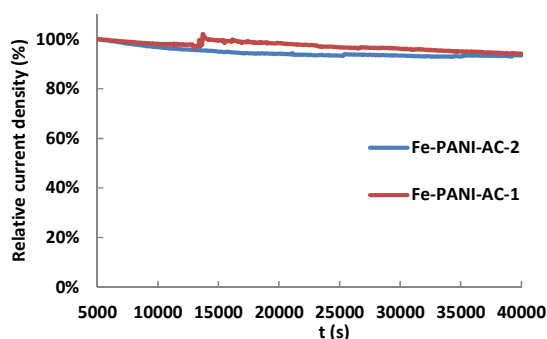
Figure 6. Relative current density vs. time ( j-t ) plot based on chronoamperometric measurements of the Fe-PANI-AC electrocatalysts at 0.01V vs. Ag/Ag 2 SO 4 in a 3 M H 2 SO 4 solution with 6% NO in the gas feed.
