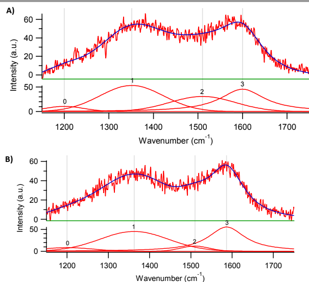
Figure 2. Deconvoluted Raman spectra of (A) Fe-PANI-AC-1 and (B) Fe-PANI-AC-2.
