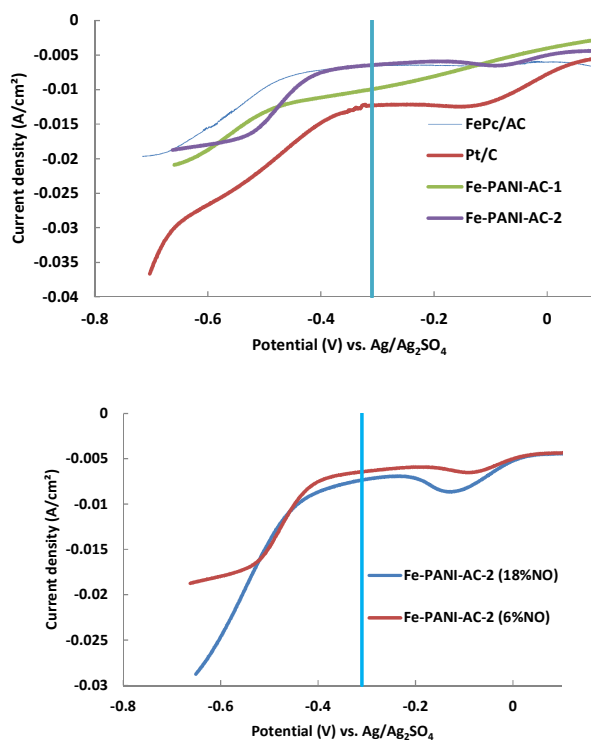
Figure 5. Top: LSV plots of the electrocatalysts under study with 6% NO in \text{N}_2 as a cathode feed. Bottom: LSV plots of Fe-PANI-AC-2 with 6 and 18% NO in the feed. The part of the plot at more negative potential relative to the standard potential for the reduction of NO to \text{NH}_2\text{OH} (marked by the vertical line at -0.31 V vs. \text{Ag}/\text{Ag}_2\text{SO}_4 ) is the region of interest for this study.
