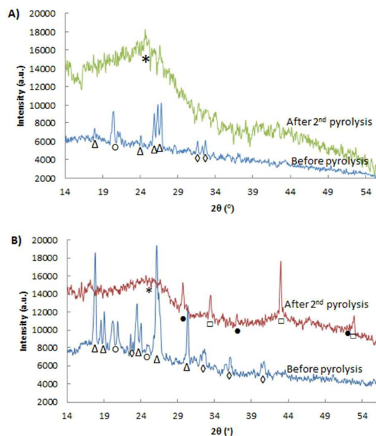
Figure 1. X-ray diffractograms of: (A) Fe-PANI-AC-1 and (B) Fe-PANI-AC-2. The peaks in the XRD pattern are identified as follows: \Delta is (\text{NH}_4)_2\text{S}_2\text{O}_8 , \diamond is \text{NH}_4\text{Cl} , \circ is polyaniline, \square is FeS, \bullet is \text{Fe}_3\text{S}_4 and * is graphitic carbon.
