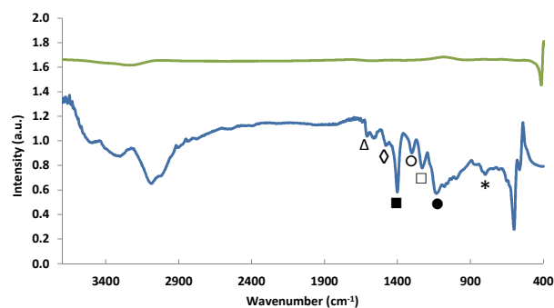
Figure 3. FT-IR spectra of Fe-PANI-AC-1 (A) before pyrolysis and (B) after the second pyrolysis.
