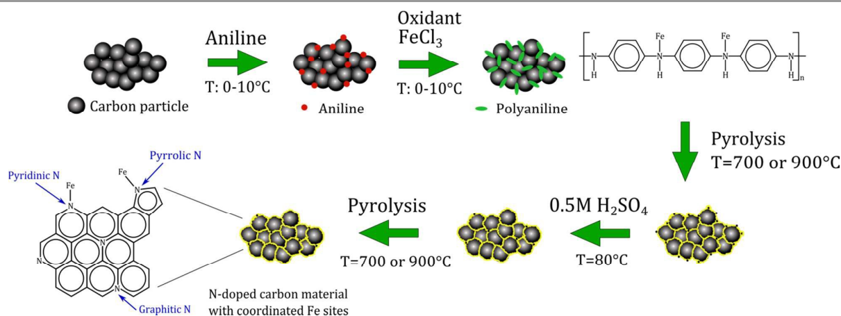
Scheme 2. Synthesis of the Fe-PANI-AC electrocatalysts.
