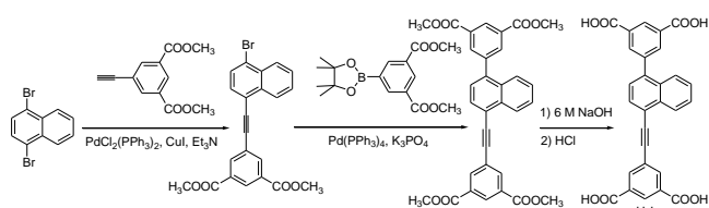
Scheme 1 Synthesis of the organic linker H_4L used to construct ZJNU-53 .
