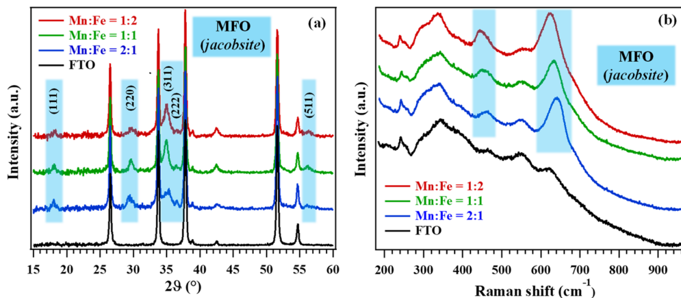
Fig. 2 (a) XRD patterns and (b) Raman spectra for MFO specimens grown on FTO from different mixtures of \text{Mn}(\text{hfa})_2/\text{TMEDA} and \text{Fe}(\text{hfa})_2/\text{TMEDA} precursors. Curves have been vertically shifted for clarity. The XRD pattern and Raman spectrum of the bare FTO substrate are also reported for comparison. In both panels, the main signals from the MFO spinel phase are highlighted by a pale blue background.
