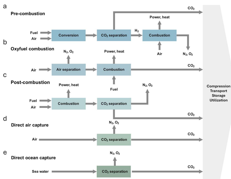
Fig. 19 General flow diagram of reactive \text{CO}_2 capture approaches: (a) pre-combustion, (b) oxy-fuel combustion, (c) post-combustion, (d) DAC, and (e) DOC. Adapted from ref. 309 with permission from Elsevier, copyright 2015.
