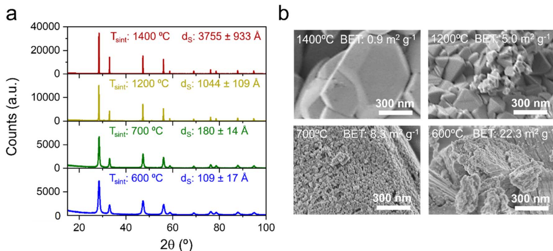
Fig. 2 Calcination temperature tunes grain size and surface area in Ce 0.9 La 0.1 O 2-δ . (a) XRD and Scherrer analysis reveal decreasing crystallite size with lower calcination temperature; and (b) FESEM images and BET analysis show strong inverse relationship between particle size and surface area.
