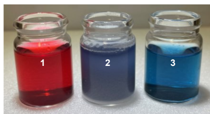
Fig. 10 Samples of red cabbage extract prepared according to the method described by James Watt. (a) Sample 1 shows extract in dilute \text{H}_2\text{SO}_4 (b) sample 2 shows extract mixed with \text{CaCO}_3 (unfiltered) and (c) sample 3 shows extract mixed with \text{CaCO}_3 and resulting \text{CaSO}_4 has been filtered off.
