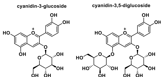
Fig. 2 Examples of glycosylated anthocyanidins.
