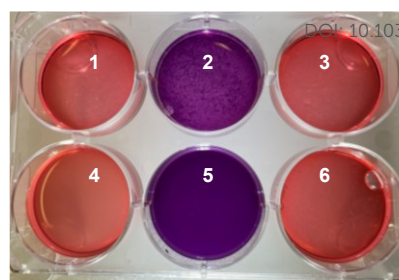
Fig. 12 Tests with pineapple juices and blackberry extracts. (a) Sample 1, blackberry extract in dilute HCl (b) Sample 2, blackberry mixed with \text{SnCl}_2 (c) Sample 3, blackberry extract (d) Sample 4, blackberry extract added to pineapple juice from a carton (e) Sample 5, blackberry extract added to pineapple juice from a tin can (f) Sample 6, blackberry extract added to fresh pineapple juice.
