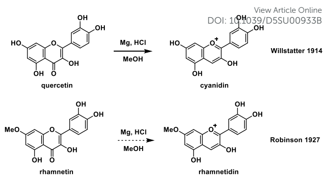
Fig. 14 Reactions of quercetin (a) and rhamnetin (b) with magnesium metal in methanolic HCl (this reaction was not successful).
