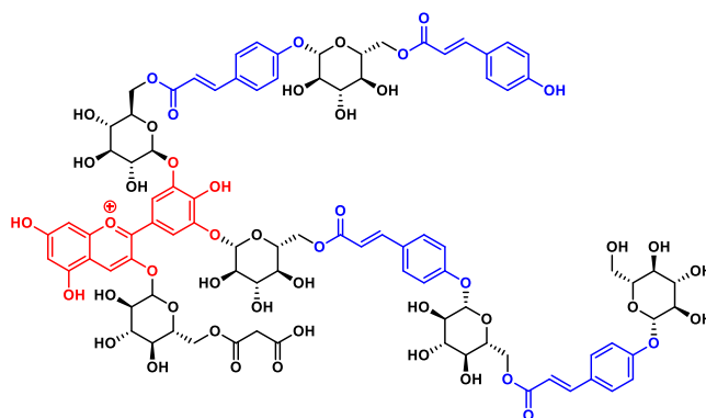
Fig. 4 Molecular structure of ternatin B1. Delphinidin is highlighted in red, acylating units are highlighted in blue and carbohydrates are shown in black.
