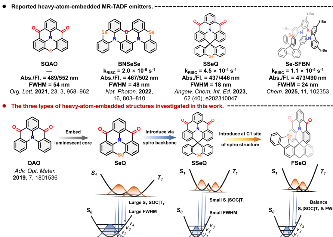
Fig. 1 Reported heavy-atom-embedded MR-TADF emitters and the three types of heavy-atom-embedded structures investigated in this work.
