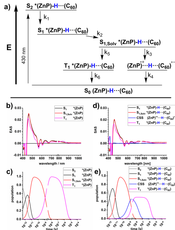
Fig. 6 (a) Analysis model used for evaluating the transient-absorption spectra of ZnP and ZnP-H \cdots C 60 . General note: Soret-band excitation results in the initial population of S_2 . Modelling the S_2 - S_1 internal conversion was necessary for a good fit. However, the long optical dispersion through the pressure cell does not allow to assign a clear EAS or SAS for S_2 . 61 (b) Evolution associated spectra (EAS) from a four exponential global analysis of ZnP in anisole at 5 MPa. 61 (c) Time profiles depicting the time-resolved population of the corresponding EAS of ZnP from global analysis. 61,62 (d) Species associated spectra (SAS) from branched six exponential target analysis of ZnP-H \cdots C 60 in anisole at 5 MPa. 61,62 (e) Time profiles depicting the time-resolved population of the corresponding SAS of ZnP-H \cdots C 60 , from target analysis. A 1000-fold excess of DMAP vs. ZnP was used in all optical spectroscopy experiments. 61,62
