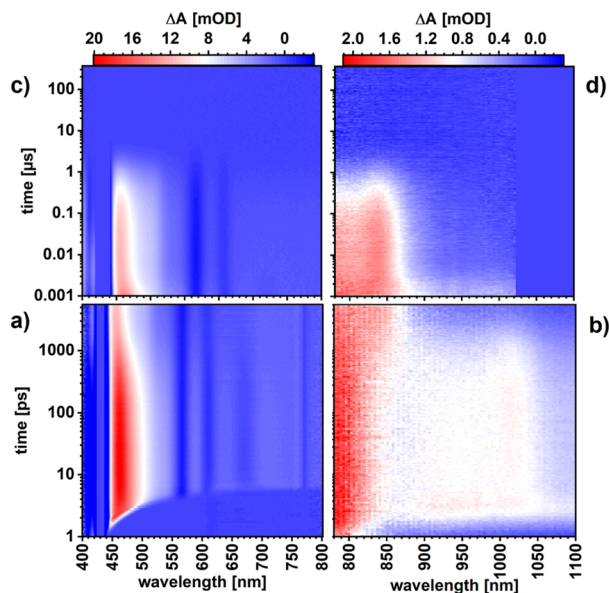
Fig. 5 fs-TAS spectra in the visible (a) and NIR region (b) of ZnP-H \cdots C 60 at 5 MPa in anisole, after photoexcitation at 430 nm with 200 nJ pulse energy. ns-TAS spectra in the visible (c) and NIR (d) under identical condition. A 1000-fold excess of DMAP vs. ZnP was used in all optical spectroscopy experiments.
