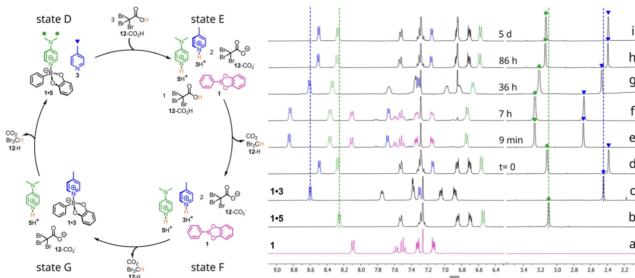
Fig. 7 Behaviour of a DL based on the B \leftarrow N bond under the action of excess ACA 12\text{-CO}_2\text{H} . Traces (a) 10 mM 1 ; (b) adduct 1·5 obtained by mixing 10 mM 1 with 10 mM 5 ; (c) adduct 1·3 obtained by mixing 10 mM 1 and 10 mM 3 ; (d) equilibrated solution of 10 mM 1 , 3 and 5 before addition of 30 mM ACA 12\text{-CO}_2\text{H} ( t = 0 ); (e–i) monitoring over time of solution in trace d after addition of ACA 12\text{-CO}_2\text{H} . \text{CDCl}_3 , 25^\circ\text{C} . Dashed vertical lines are guides for the eye. On each spectrum, the relevant signals for 1 are marked in pink, those of 3 in blue, while those of 5 are coloured in green.
