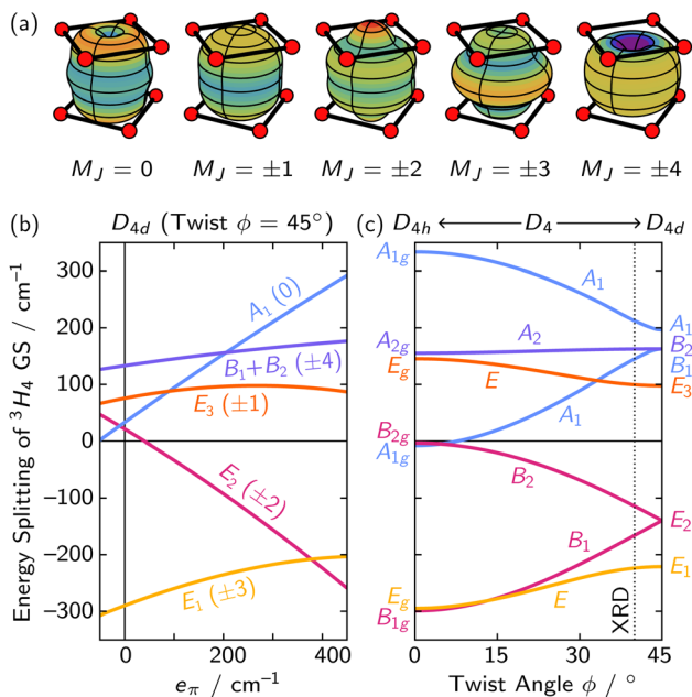
Fig. 3 (a) Charge density distributions for the M_J levels within the {}^3H_4 GS of \text{Pr}^{\text{III}} show the \pm 3 levels should be lowest in energy. (b) The predicted splitting from an AOM treatment of 1\cdot\text{Pr} in perfect D_{4d} symmetry using e_\sigma = 400 \text{ cm}^{-1} . (c) Deviations from ideal D_{4d} symmetry ( 45^\circ twist) cause descent into D_4 symmetry. Notably, this splits the E_2 level into a B_1 and a B_2 level ( e_\sigma = 400 \text{ cm}^{-1} , e_\pi = 265 \text{ cm}^{-1} ).
