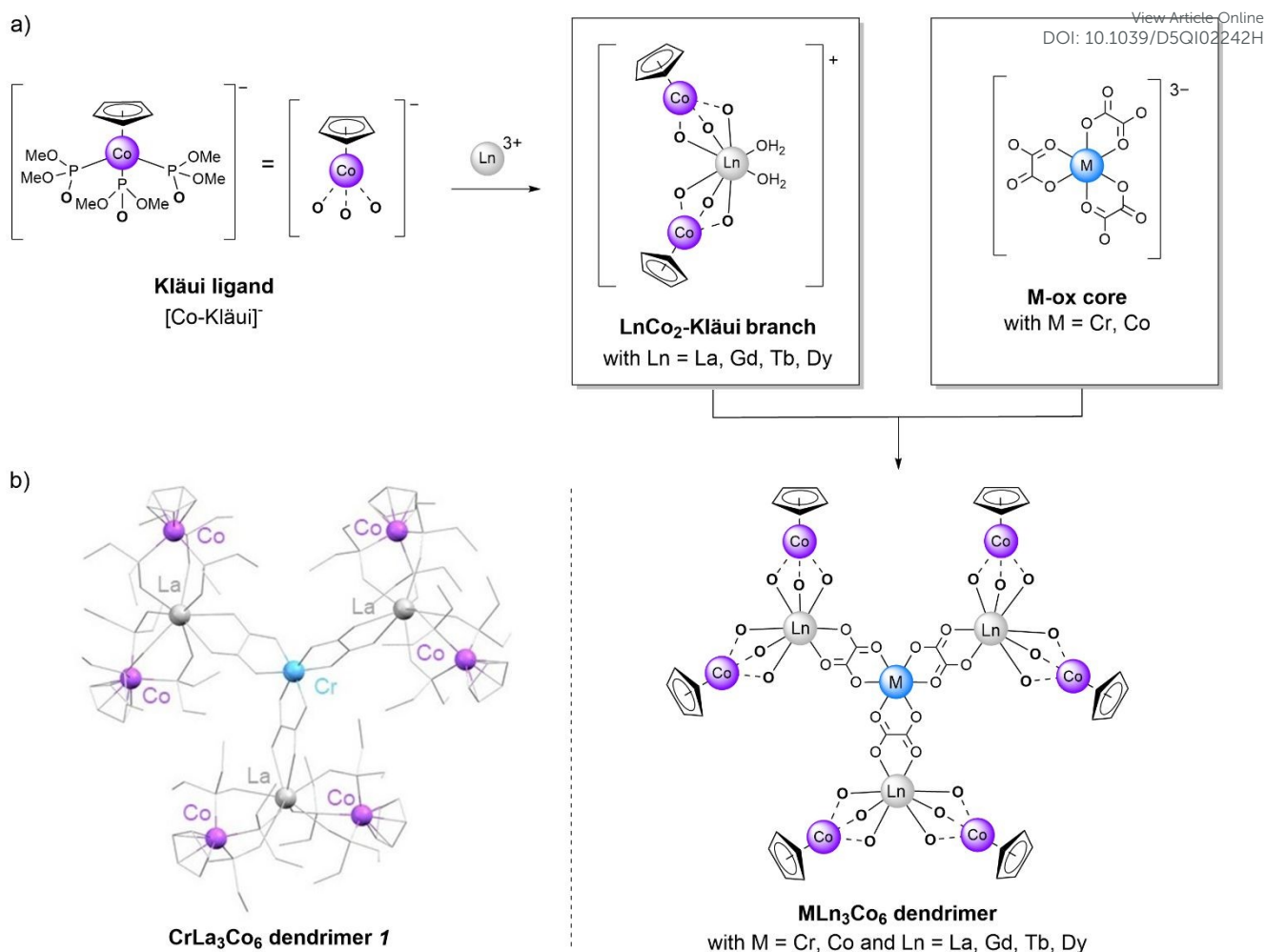
Figure 1. a) Convergent synthesis using a modular approach yielding the hetero-trimetallic dendrimers topology MLn 3 Co 6 (M = Cr, Co and Ln = La, Gd, Tb, Dy); b) Crystallographic representation of the decanuclear complex CrLa 3 Co 6 1 . CCDC 2451819. Only metal ions are coloured while hydrogen atoms and solvent molecules are omitted for clarity.
