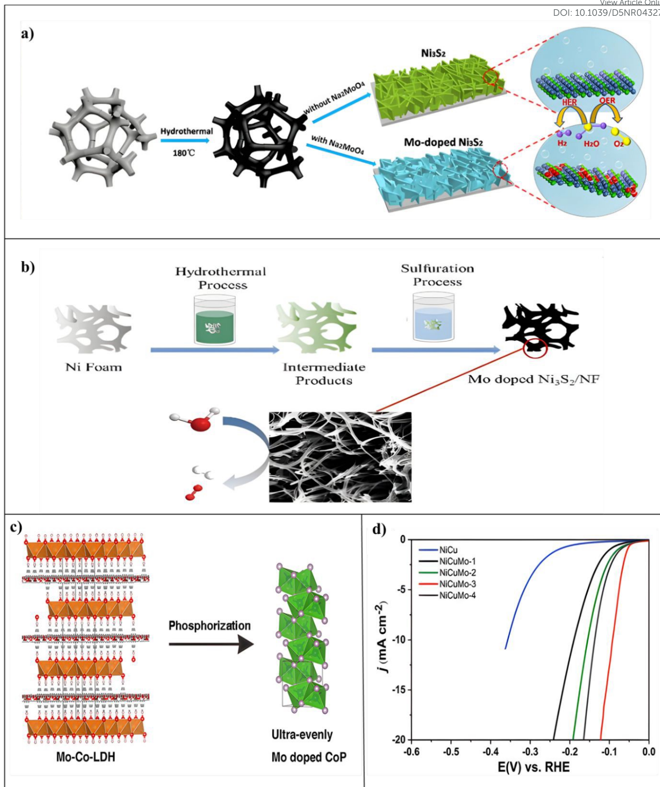
Figure 9. (a) A demonstration of the Mo-doped Ni 3 S 2 nanosheet design. reproduced from Ref. [96] with permission. Copyright 2018, Elsevier. (b) On nickel foam (NF) a 3D Mo-doped Ni 3 S 2 nanowire network was successfully produced using a hydrothermal and sulfidization process. reproduced from Ref. [103] with permission. Copyright 2018, Wiley. (c) Diagrammatic Representation of Ultra-Even Mo-Doped CoP Composite Formation. reproduced from Ref. [101] Copyright 2021, ACS. (d) NiCu and NiCuMo catalysts electrocatalytic HER performance in 0.5 M H 2 SO 4 . reproduced from Ref. [98] Copyright 2019, RSC.
