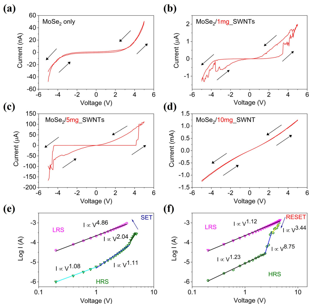
Fig. 3 I - V curves showing the emergence of memristive behaviour with increasing SWNT content, confirming the role of the hybrid structure in nonlinear conduction. (a) I - V curve for pure MoSe 2 , (b) I - V curve for MoSe 2 with 1 mg of SWNTs showing the emergence of a counter-clockwise hysteresis loop (arrows indicate the sweep direction), (c) I - V curve for MoSe 2 with 5 mg of SWNTs exhibiting enhanced resistive switching, (d) I - V curve for MoSe 2 with 10 mg of SWNTs displaying near-linear behaviour, (e) log-log plot of the SET transition for the 5 mg device (from c), and (f) log-log plot of the RESET transition for the 5 mg device (from c), both confirming SCLC conduction mechanisms.
