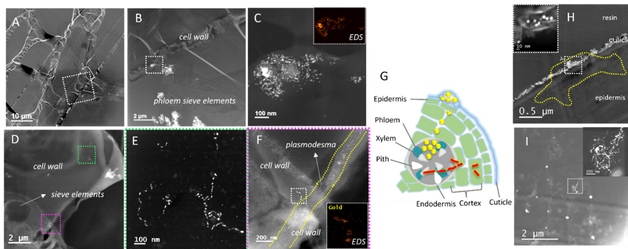
Fig. 6 HAADF-STEM images of Au nanocarriers in eggplant stems: (A–C, H) show spherical nanocarriers, and (D–F, I) show wire-shaped nanocarriers. (G) A schematic drawing illustrating the distribution of nanocarriers in plant stems. White dotted boxes in (A, B, F, H, and I) are magnified to highlight regions containing nanocarriers, while yellow dotted lines mark areas with nanocarriers. Green and purple dotted boxes in (D) indicate regions of interest, which are further magnified in (E) and (F).
