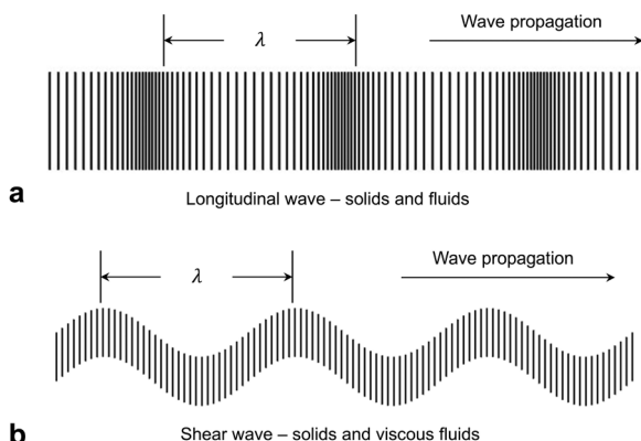
Fig. 7 Ultrasound wave modes classification: (a) compressional (longitudinal) wave, whose particle motion is parallel to the wave propagation direction and (b) shear wave, whose particle motion is perpendicular to the wave propagation.
