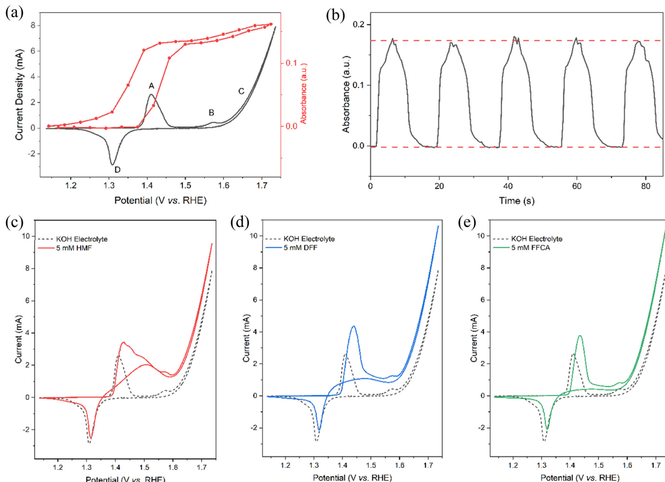
Fig. 6 Electrochemical redox characteristics of electrodeposited \text{Ni(OH)}_2 . (a) Overlay of the synchronous CV scan and the corresponding in situ UV-vis profile ( \lambda = 570 \text{ nm} ) measured in 1 M KOH. (b) Absorbance profile recorded over the last 5 cycles of an extended 20-cycle CV measurement. CV measurements recorded with (coloured) and without (black) the addition of 5 mM (c) HMF, (d) DFF, and (e) FFCA. Scan rate = 20 \text{mV s}^{-1} .
