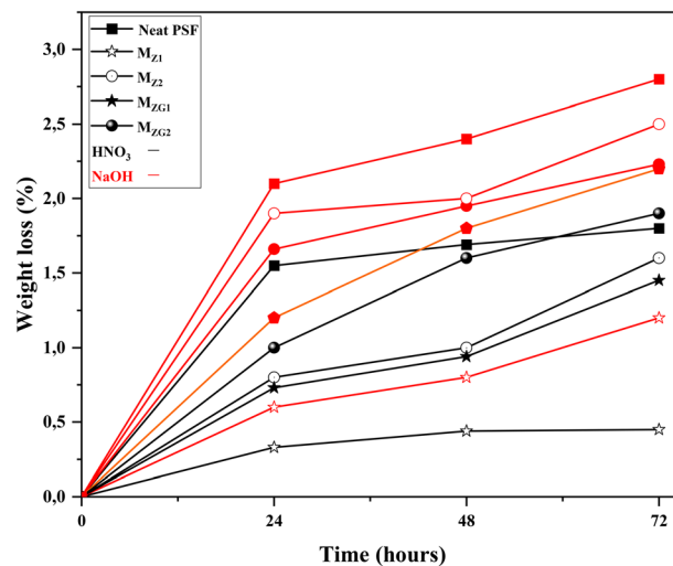
Fig. 10 Weight loss percentage versus time of the prepared membranes after immersion in \text{HNO}_3 (0.2 M) and NaOH (0.5 M) for 3 days.
