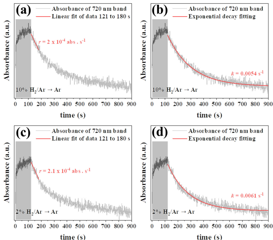
Fig. 4 Effect of \text{H}_2 partial pressure on the BAS formation and decomposition on the 4 W-1Pt/SiO 2 catalyst. (a) The BAS decomposition rate r_{\text{d(BAS)}} , and (b) BAS decomposition rate constant ( k_{\text{d(BAS)}} ) after removal of 10% \text{H}_2/\text{Ar} . (c) The BAS decomposition rate r_{\text{d(BAS)}} , and (d) BAS decomposition rate constant ( k_{\text{d(BAS)}} ) after removal of 2% \text{H}_2/\text{Ar} . The cycle duration is 900 s, where \text{H}_2/\text{Ar} was introduced for the first 120 s and pure Ar for the remaining 780 s. The r_{\text{d(BAS)}} was calculated by taking a linear approximation of between 121 and 180 s (60 s duration after \text{H}_2 removal) and k_{\text{d(BAS)}} was calculated by exponential decay fitting of absorbance data from 121 to 900 s. All catalysts were pre-reduced at 673 K in 10% \text{H}_2/\text{Ar} for 60 minutes. All experiments were conducted at 423 K.
