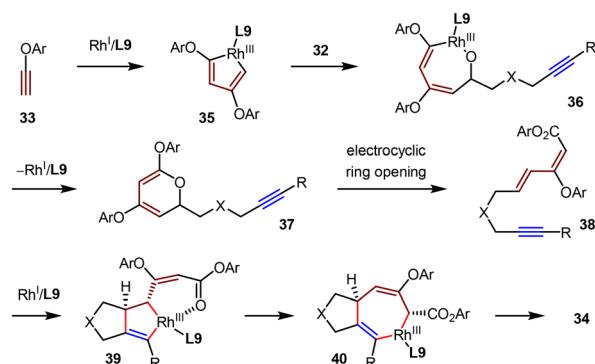
Scheme 12 Rh(I)/(R)-H 8 -BINAP-catalyzed intermolecular [2+2+2] trimerization/asymmetric intramolecular [4+2] cycloaddition.
