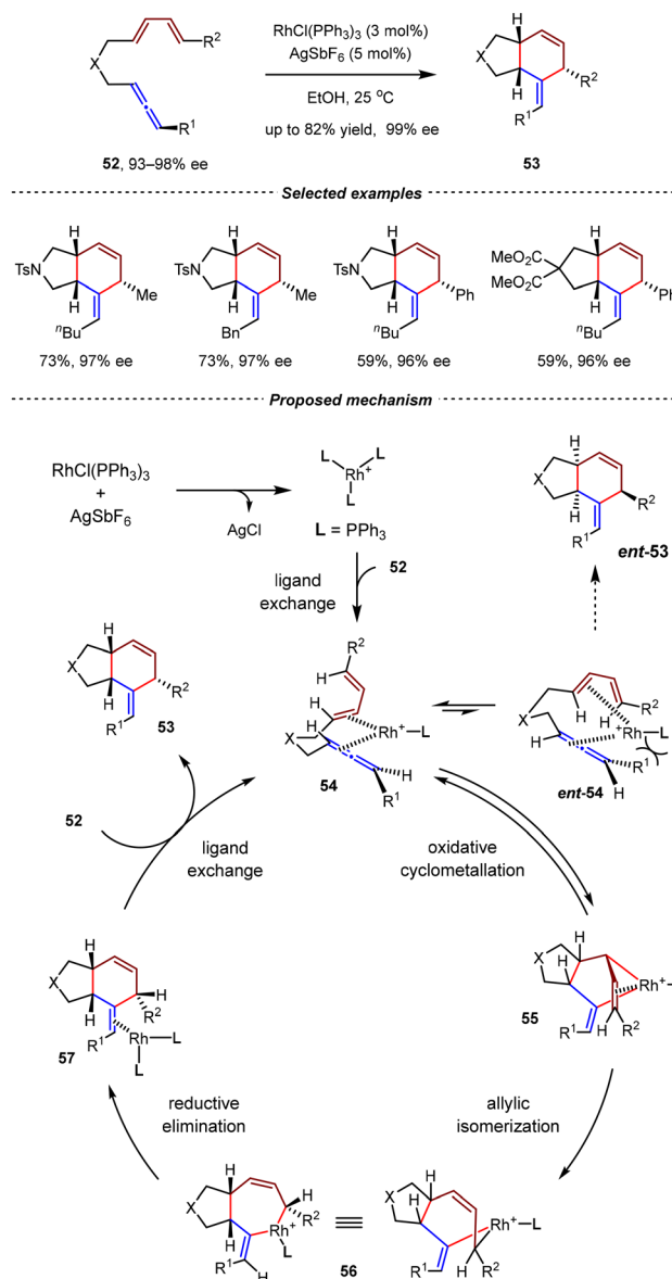
Scheme 16 \text{Rh}(\text{PPh}_3)_3\text{SbF}_6 -catalyzed intramolecular [4+2] cycloadditions of optical active allene-1,3-dienes.
