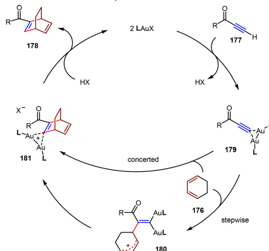
Scheme 39 Au(I)/phosphoramidite-catalyzed asymmetric intermolecular [4+2] cycloadditions of ynones and cyclohexa-1,3-dienes.
