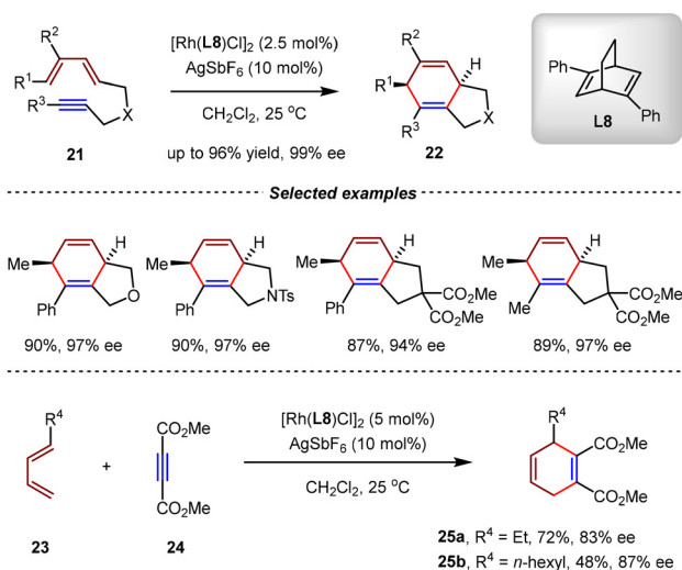
Scheme 10 Rh(I)/chiral diene-catalyzed asymmetric intramolecular and intermolecular [4+2] cycloadditions.
