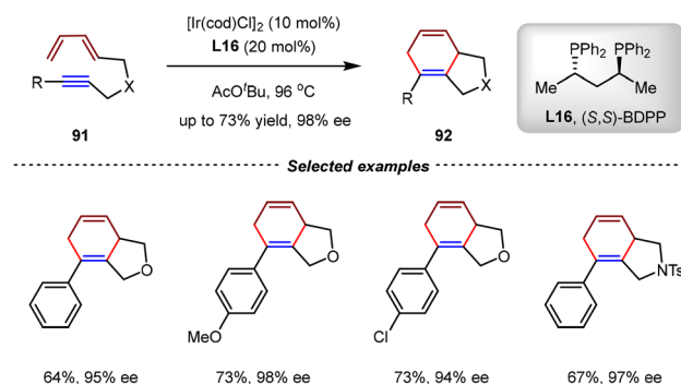
Scheme 23 Ir(III)/BDPP-catalyzed asymmetric intramolecular [4+2] cycloaddition of diene-yne.
