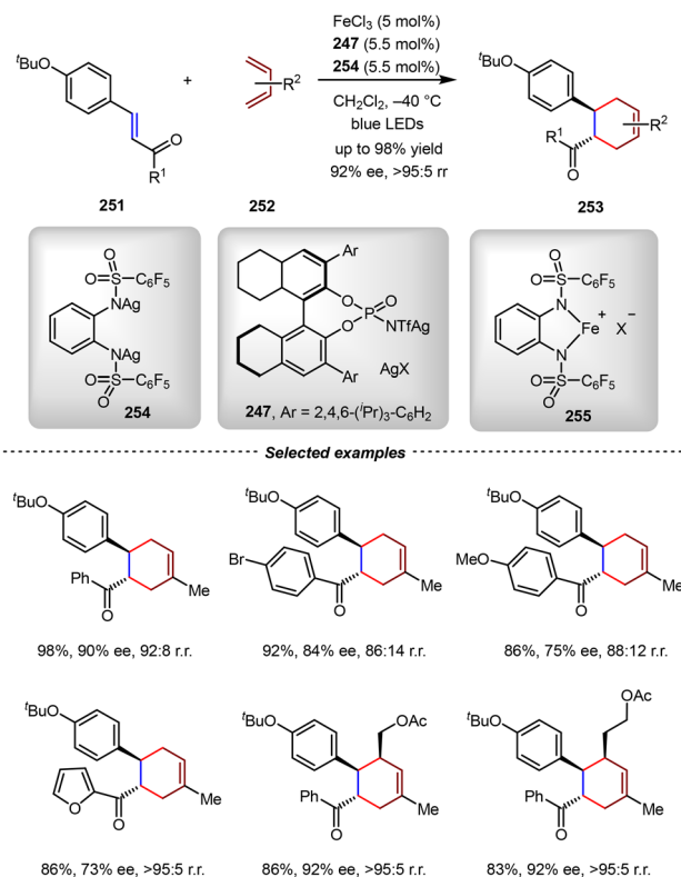
Scheme 51 A new Fe(III) photocatalyst consisting of a chiral phosphoramidate anion and an achiral bidentate ligand.
