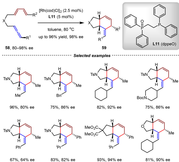
Scheme 17 Rh(I)/dppeO-catalyzed intramolecular [4+2] cycloadditions of optically active allenyl 1,3-dienes.
