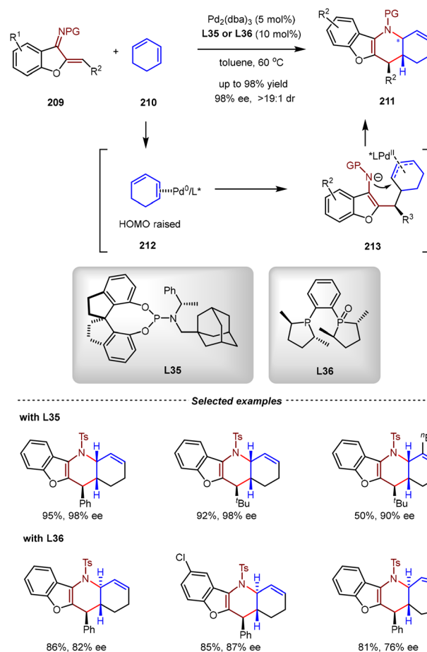
Scheme 44 Pd(0)-catalyzed formal inverse-electron-demand aza-Diels–Alder reactions between 1,3-cyclohexadiene and aurone-derived 1-azadienes.
