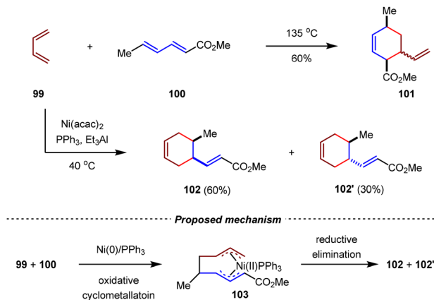
Scheme 25 Ni(0)/PPh 3 -catalyzed cross-[4+2] cycloadditions of 1,3-butadiene with methyl sorbate.
