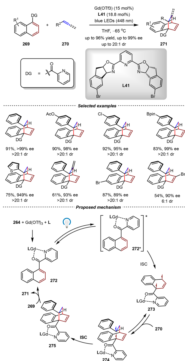
Scheme 54 Gd(III)-catalyzed asymmetric [4+2] photocycloadditions of naphthalenes and styrenes.
