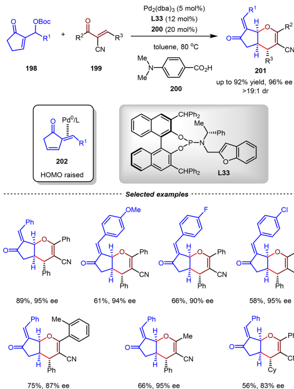
Scheme 42 Pd(0)-catalyzed asymmetric inverse-electron-demand oxa-Diels–Alder reactions of MBH carbonates and \alpha -cyano chalcones.
