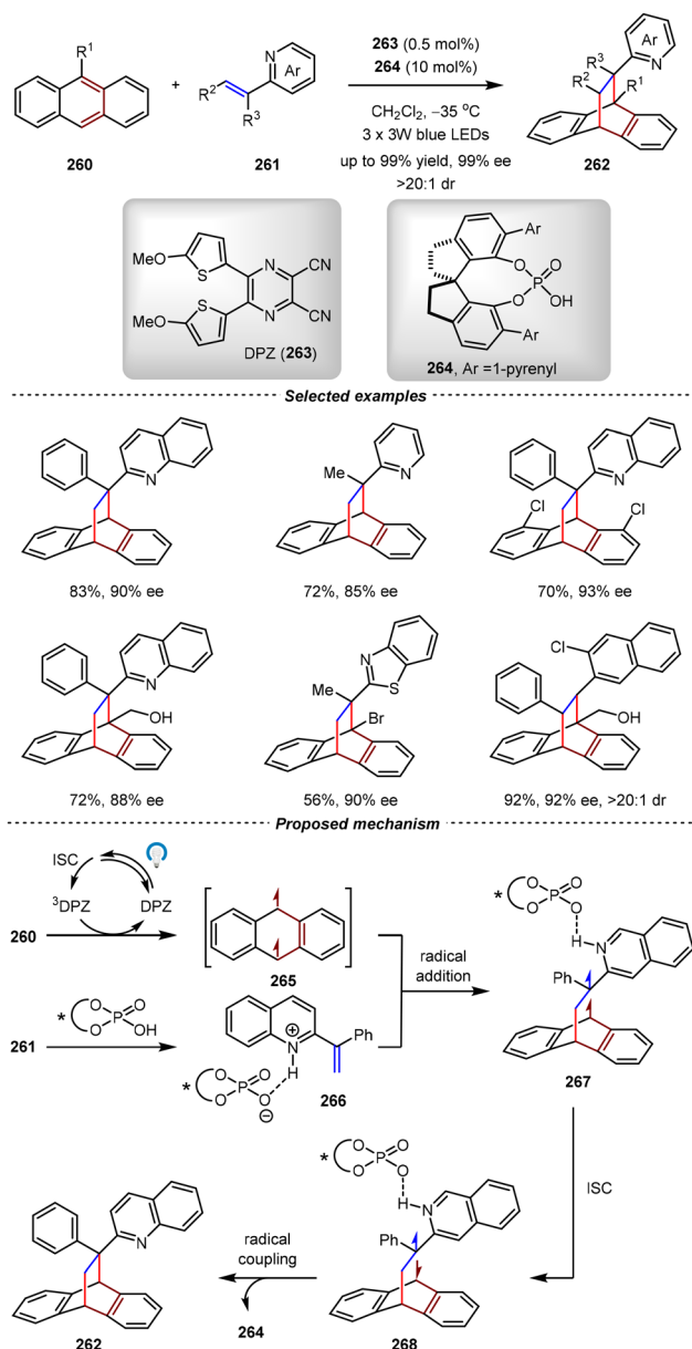
Scheme 53 Asymmetric [4+2] dearomative photocycloadditions of anthracene with alkenylazaarenes.
