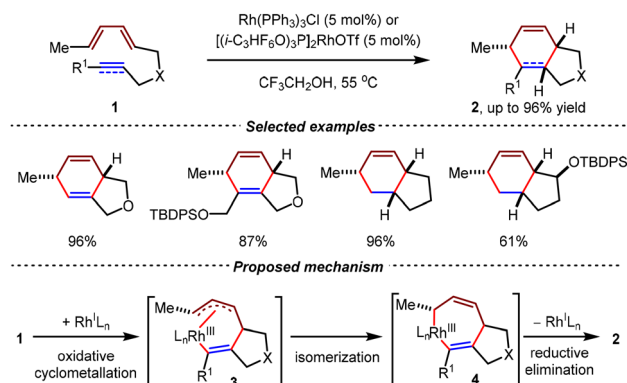
Scheme 4 Rhodium(I)-catalyzed intramolecular [4+2] cycloadditions of diene-ynes and trienes.
