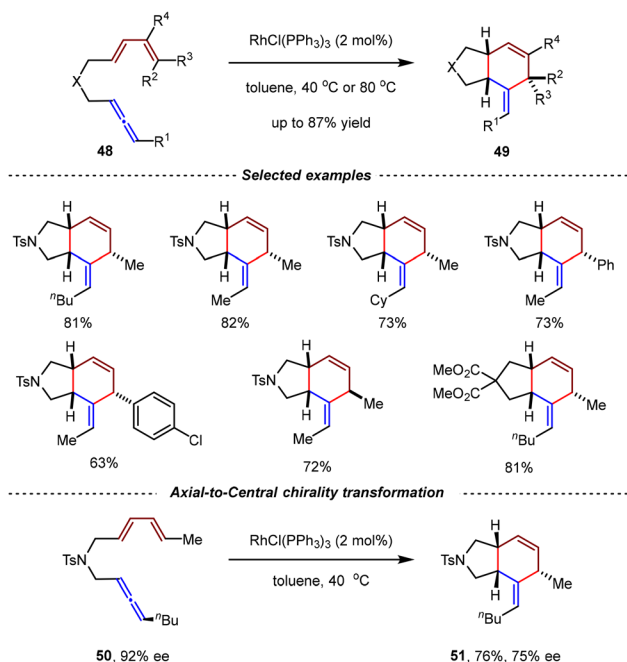
Scheme 15 \text{RhCl}(\text{PPh}_3)_3 -catalyzed intramolecular [4+2] cycloadditions of 1,3-disubstituted allene-1,3-dienes.
