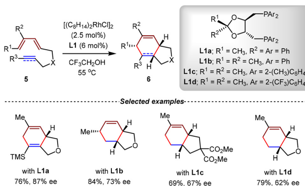
Scheme 5 Rhodium(I)-catalyzed asymmetric intramolecular [4+2] cycloadditions of diene-ynes and trienes.
