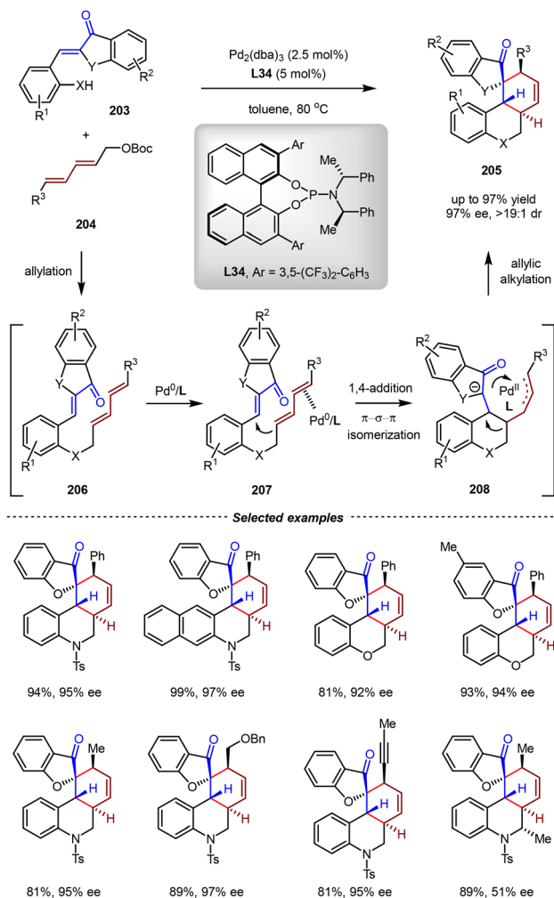
Scheme 43 Pd(0)-catalyzed tandem asymmetric Tsuji–Trost allylation and intramolecular [4+2] cycloaddition reactions.
