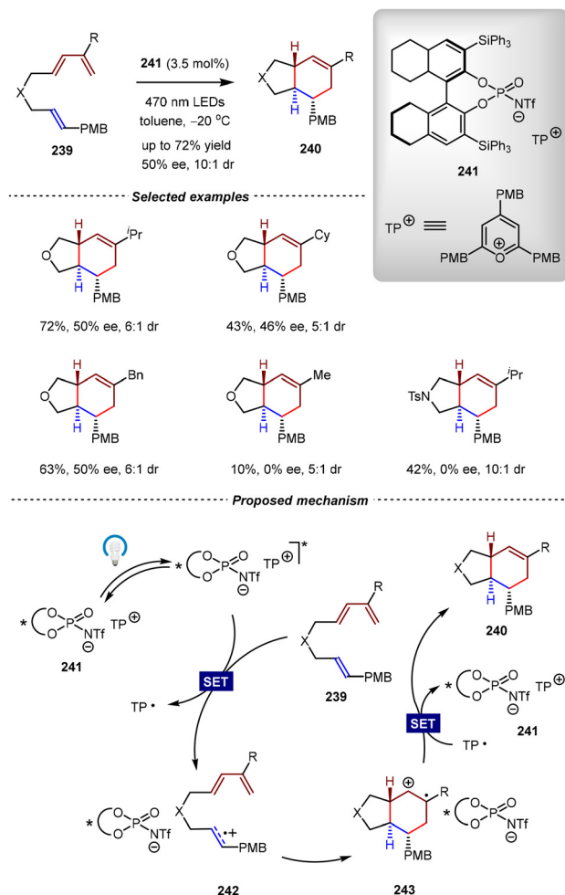
Scheme 49 Cationic oxopyrylium-catalyzed asymmetric radical cation intramolecular [4+2] cycloadditions of unactivated diene-ene.
