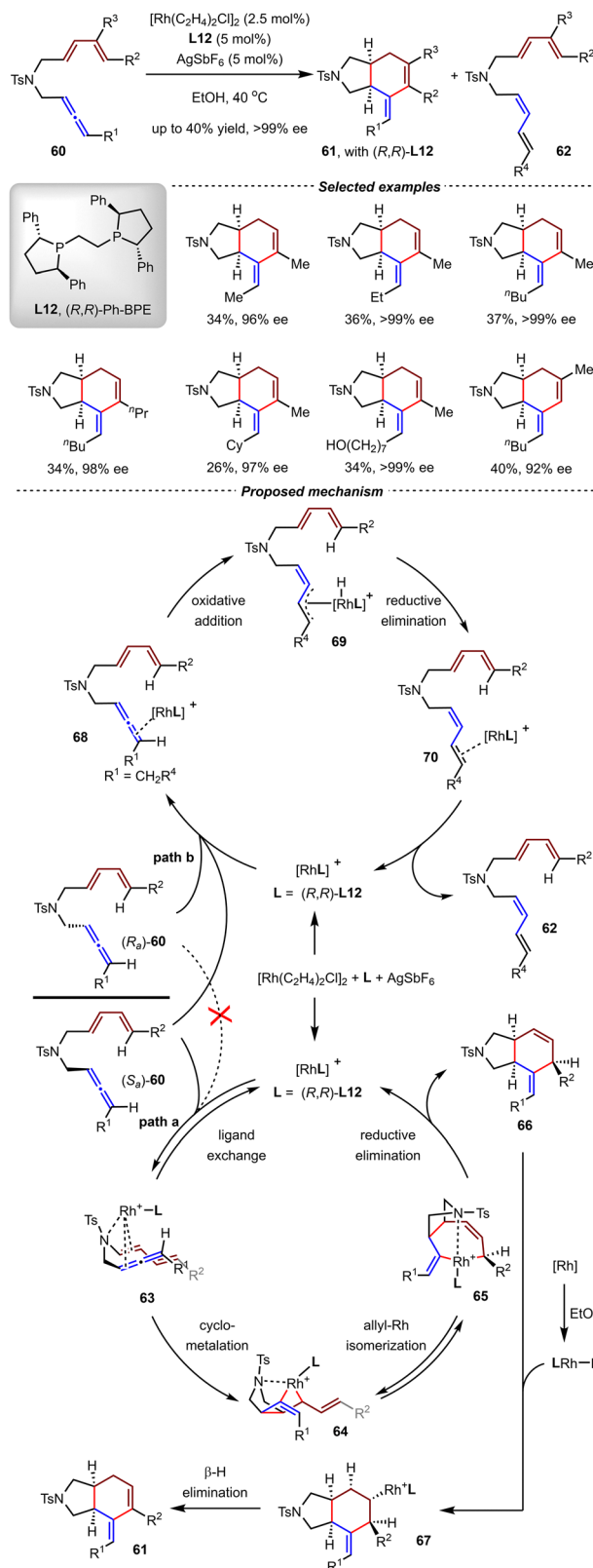
Scheme 18 Rh(I)/Ph-BPE-catalyzed kinetic resolution of racemic 1,3-disubstituted allene-1,3-dienes.
