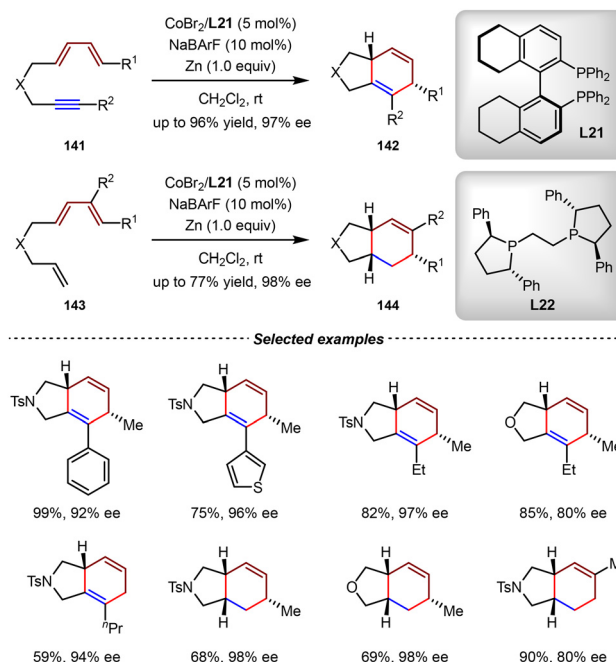
Scheme 31 \text{Co}(\text{I}) -catalyzed intramolecular [4+2] cycloaddition reactions of unactivated diene-yne and trienes.
