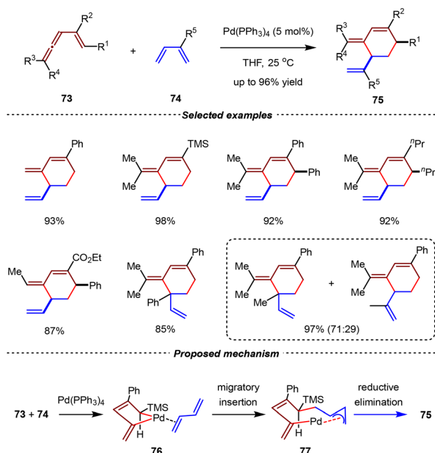
Scheme 20 \text{Pd}(\text{PPh}_3)_4 -catalyzed intermolecular [4+2] cycloadditions of vinylallenes and 1,3-dienes.
