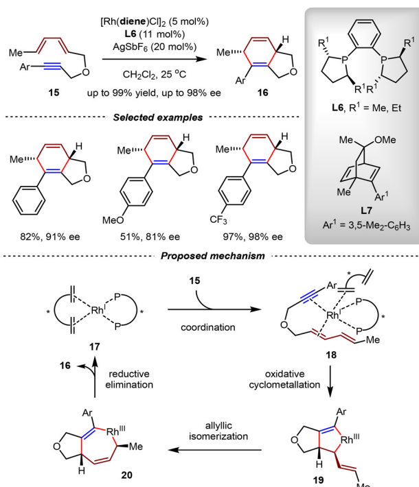
Scheme 9 Asymmetric intramolecular [4+2] cycloadditions catalyzed by a rhodium(i)/DUPHOS/diene complex.
