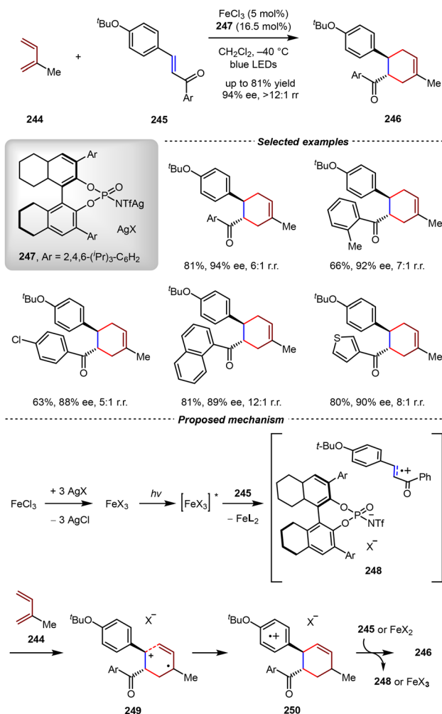
Scheme 50 Asymmetric radical cation [4+2] cycloadditions catalyzed by the combination of FeCl 3 and silver N -triflylphosphoramidate.
