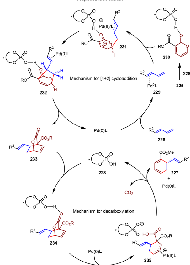
Scheme 47 Pd(0)/chiral phosphoric acid co-catalyzed periselective and enantioselective cross-[4+2] cycloaddition and decarboxylation reactions.
