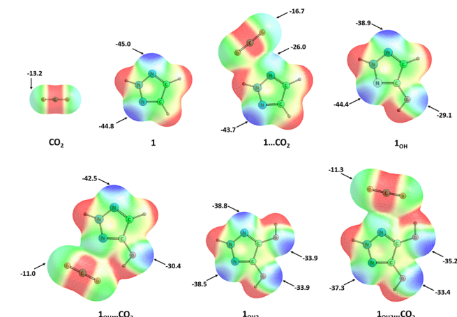
Fig. 3 MESP on the 0.005 a.u. isodensity surface for CO 2 , 1 , 1OH , 1OH 2 , and their CO 2 complexes. V_{\min} values (kcal mol -1 ) and N...C, O-H...O distances (Å) at the M06-2X/cc-pVQZ level of theory. Color gradient: blue (electron-rich) to red (electron-deficient).
