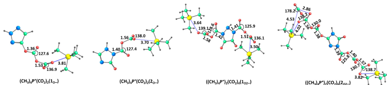
Fig. 10 Representative structures of triazolate- \text{CO}_2 adducts in ethanol with tetramethylphosphonium counter-ions, computed at the M06-2X/SMD/cc-pVTZ level. Distances in Å, angles in degrees; Color key: gray – H, blue – N, green – C, red – O, yellow – P.
