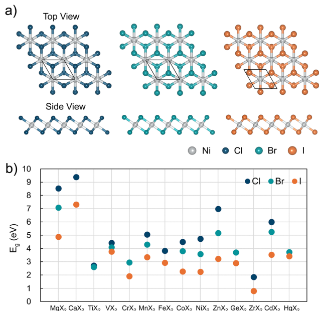
Fig. 4 Compositional dependence of bandgap values on halogen elements in \text{MX}_2 monolayer compounds. (a) An example of optimized \text{NiX}_2 where X is exchanged among Cl, Br, and I. (b) Dependence of bandgap values.
