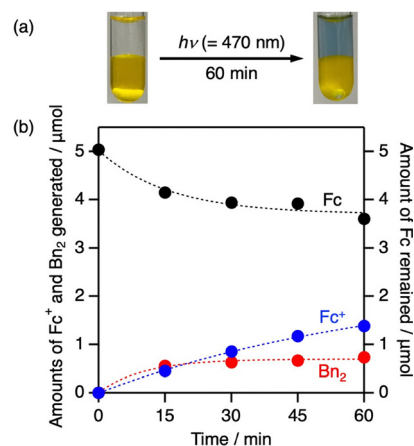
Fig. 2 (a) Photographs of a biphasic solution before and after irradiation, and (b) time course of \text{Fc}^+ / \text{Bn}_2 formation and Fc consumption along with Fc conversion from a biphasic \text{H}_2\text{O}/\text{DCE} solution (1:1, v/v; 2.0 mL) containing Fc (5.0 mM, 5 μmol), Ir (0.05 mM, 50 nmol), and Bn–Br (50 mM, 50 μmol) under visible-light irradiation ( \lambda = 470 \text{ nm} ).
