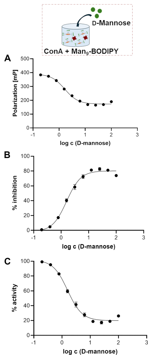
Fig. 6 Binding curves (A–C) of the competitive FP assays using fixed concentrations of Man 9 -BODIPY (0.5 \mu\text{M} ) and ConA (2 \mu\text{M} ) and adding increasing concentrations of D-mannose. The fluorescence polarization is expressed in millipolarization (mP) units (A). The relationship between relative inhibition (%), activity (%), and \log c (D-mannose) is also shown. Relative inhibition refers to competitive inhibition of Man 9 -BODIPY binding to ConA normalised to the maximum absolute inhibition achieved, while relative activity refers to the values describing relative Man 9 -BODIPY binding to ConA.
