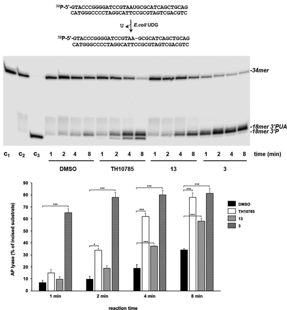
Fig. 4 Effect of compounds 3 and 13 on the AP-lyase activity of hOGG1 on 8oxoG:C-containing DNA. Upper panel: PAGE gel after autoradiographic readout. The assay was performed using 1 nM of the [ 32 P]5'-labeled uridin-containing substrate, previously treated with 0.2 U of E. coli UDG to obtain a natural AP site, incubated with 10 nM hOGG1, 20 mM EDTA and either 10% DMSO or 6.25 \mu M TH10785, 20 \mu M 13 and 20 \mu M 3 . After incubation for the indicated times at 37 ^{\circ} C, reactions were stopped and samples further analyzed by 7 M urea-20% PAGE and autoradiography. C 1 : control of no UDG-treated DNA incubated for 8 min at 37 ^{\circ} C; C 2 : control of UDG treated DNA incubated for 8 min at 37 ^{\circ} C; C 3 : alkaline degradation of the UDG treated DNA. Lower panel: bar chart of the AP lyase activity ( n = 3 ; means \pm SEM). Significance of the results was determined with a two-tailed paired t -test. * P < 0.05 ; P < 0.01 ; *** P < 0.001 . 3'-PUA – 3' phospho unsaturated aldehyde. Structures of compounds 3 and 13 depicted in Table 1.
