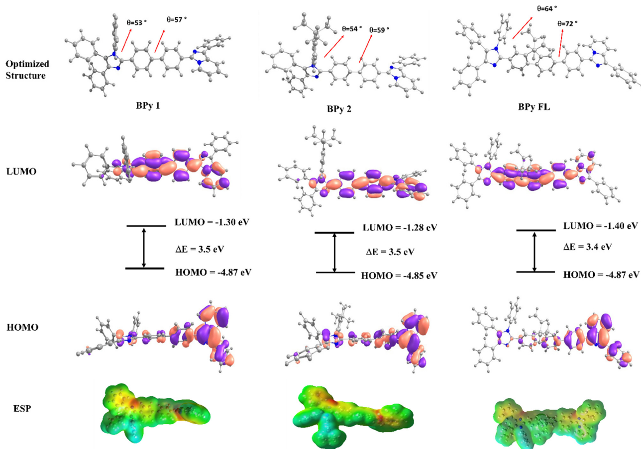
Fig. 3 Optimized molecular geometry, HOMO/LUMO energy levels, and electrostatic potential map of the fluorophores of BPpy-1 , BPpy-2 and BPpy-FL .
