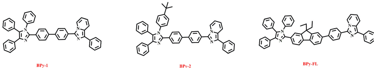
Fig. 2 Chemical structures of the synthesized fluorophores.
