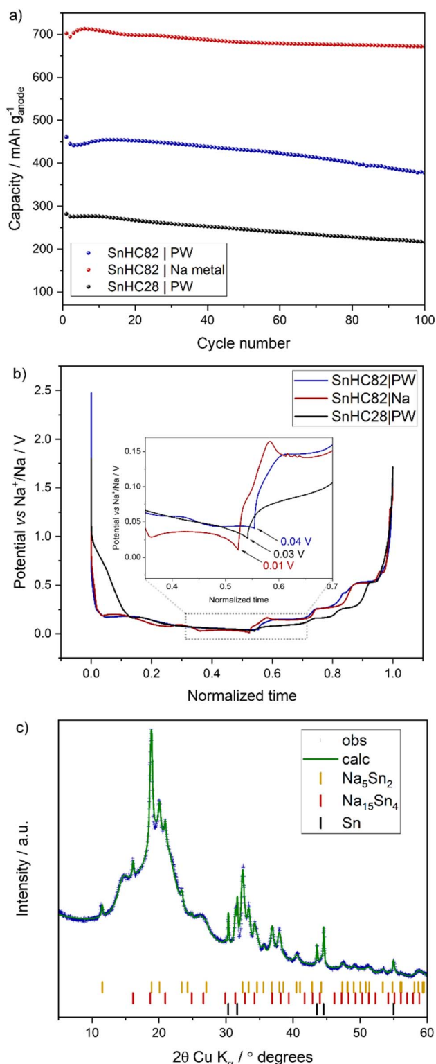
Fig. 8 (a) Charge capacity per grams of anode for SnHC82 and SnHC828 cycled in full-cells containing PW cathode (N/P of 1.1) and for SnHC82 cycled in Na half-cell. (b) First cycle anode voltage profile for SnHC82 and SnHC828 in full cells (obtained from three electrodes cell test) with PW as cathode and SnHC82 in half-cell (coin cell). (c) Ex situ XRD of the SnHC82 electrode extracted from the full-cell after a full charge (sodiation) at 50 mA g -1 .
