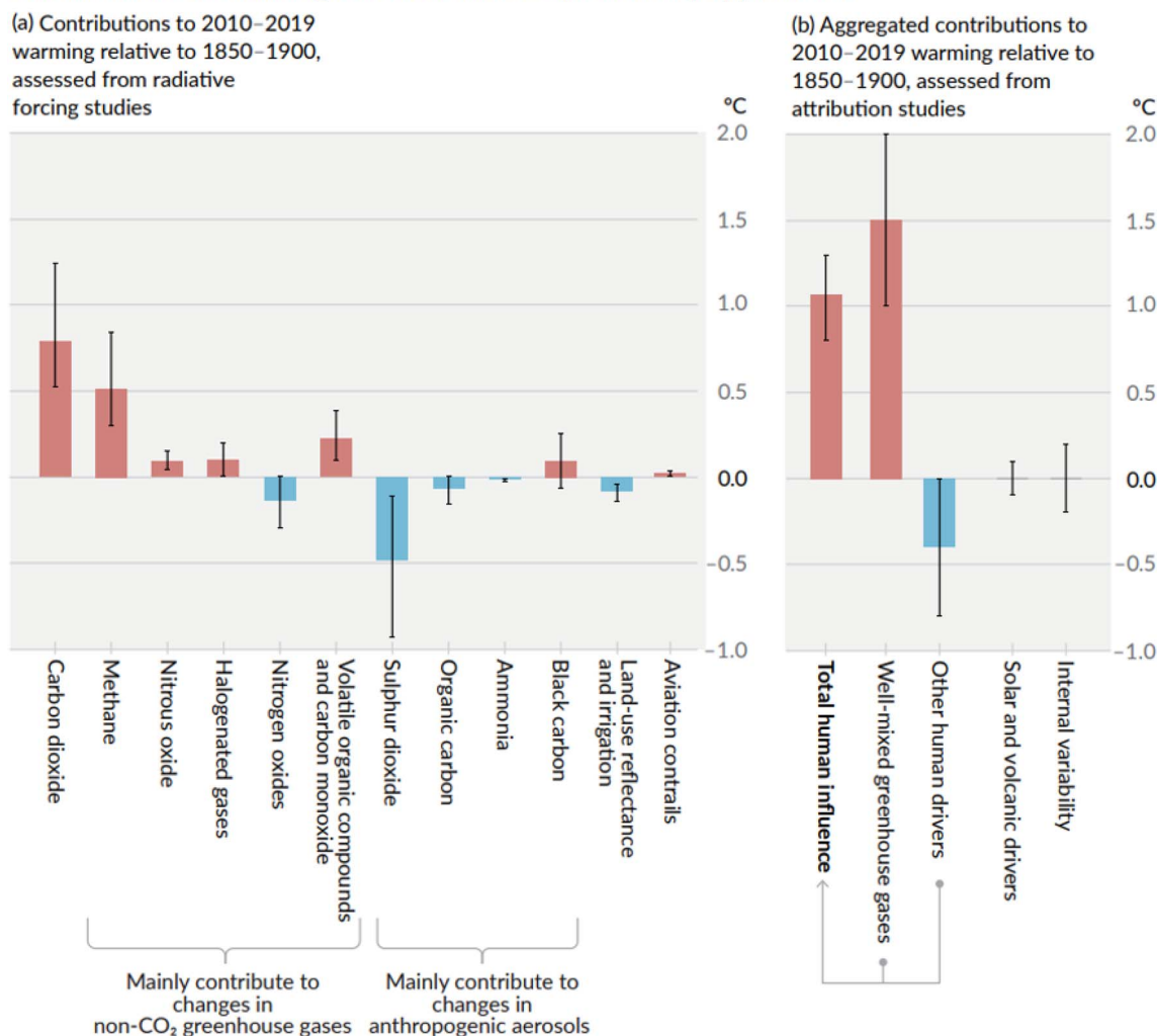
Fig. 1 Comparison of the effect of climate forcers on global warming as assessed by the IPCC AR6 report (2021), 3,4 showing the significant contributions of carbon dioxide and methane to global warming.
