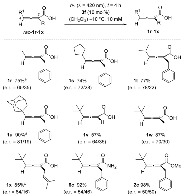
Scheme 4 Influence of substitution and binding motif on the outcome of the photochemical deracemization of 2,3-allenoic acids rac -1r to rac -1x and of allenoic acid derivatives rac -6c and rac -2c. a Yield and e.r. of the product were obtained after methyl ester formation as described in Scheme 2. b Yield of the isolated carboxylic acid, the e.r. was determined after primary amide formation.
