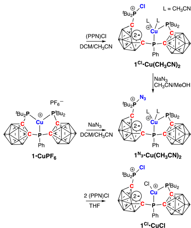
Scheme 5 Ligand-centered reactivity of [\text{tBuP-closo-}\{\text{C}_2\text{B}_{10}\}\text{-PhP-closo-}\{\text{C}_2\text{B}_{10}\}\text{-tBuP}]\text{CuPF}_6 ( 1\cdot\text{CuPF}_6 ) with chloride and azide anions. Unlabeled cluster vertices represent BH units.
