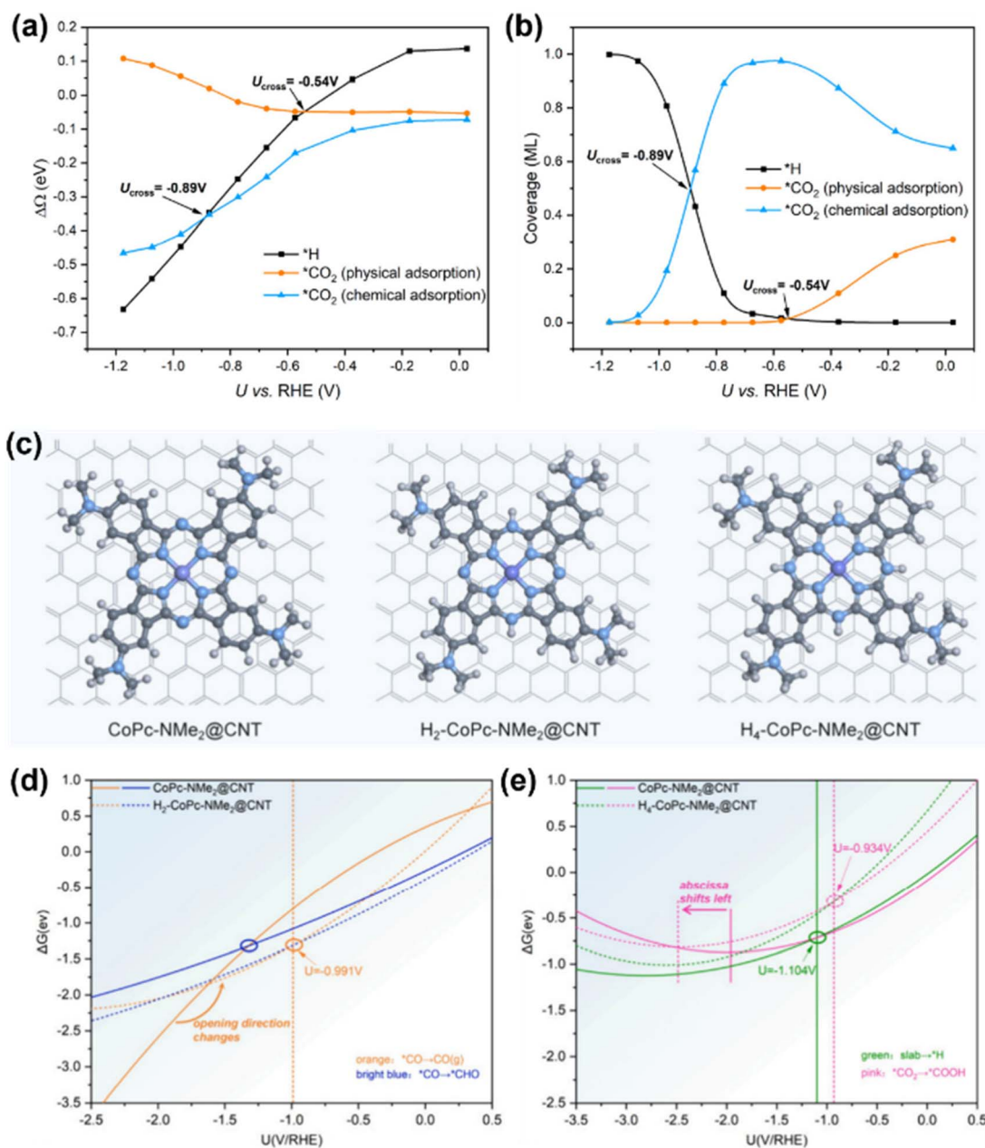
Fig. 9 (a) Potential-dependent reaction energetics of physical and chemical adsorption of CO 2 and ^*H formation on CoPc. (b) Potential-dependent competition of coverages among physical and chemical adsorption of CO 2 and ^*H formation on CoPc. 105 (c) Structural illustration of CoPc-NMe 2 @CNT, H 2 -CoPc-NMe 2 @CNT and H 4 -CoPc-NMe 2 @CNT. (d) and (e) Curves of Gibbs free energy change ( \Delta G ) for the key steps determining the potential for maximum MeOH selectivity for CoPc-NMe 2 @CNT, H 2 -CoPc-NMe 2 @CNT and H 4 -CoPc-NMe 2 @CNT as a function of applied potential. 106 Reproduced from ref. 105 and 106 with permission from American Chemical Society, copyright 2023, 2024.
