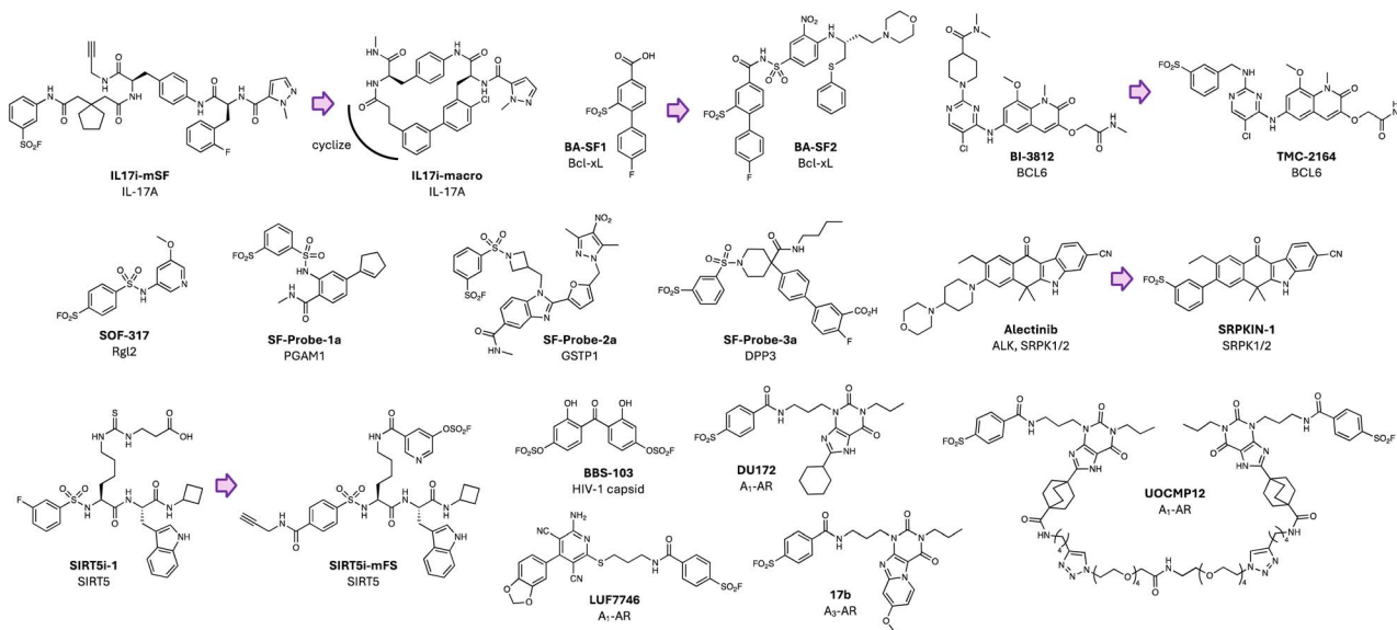
Fig. 3 Tyrosine-targeting covalent chemical probes employing sulfonamide exchange warheads.
