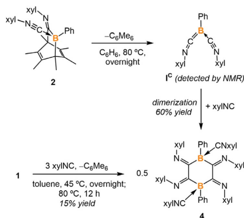
Scheme 2 Synthesis of the tetraiminylnyl-1,4-diboracyclohexane 4 .
