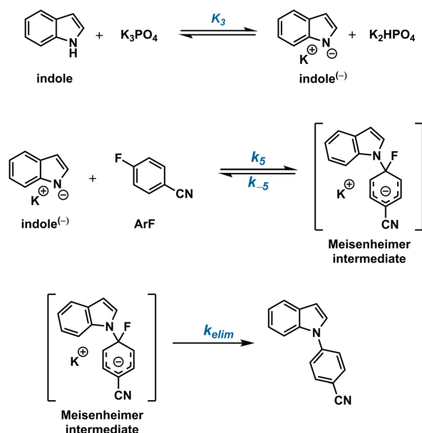
Scheme 4 Mechanisms for specific-base-catalysed concerted/borderline and stepwise S_N\text{Ar} .
