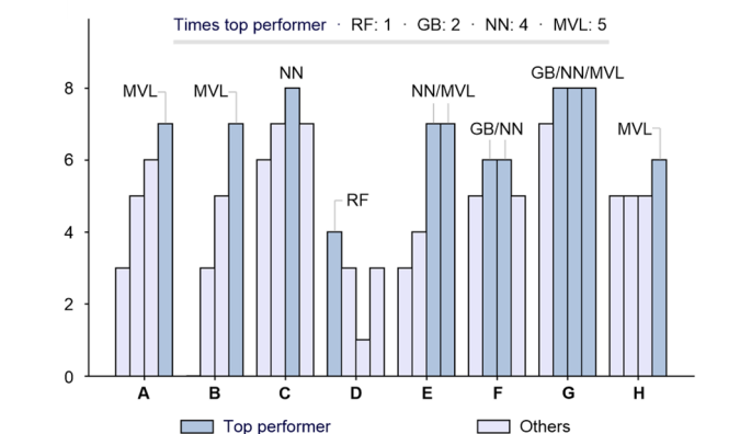
Fig. 4 (A) Calculation of the updated ROBERT score. (B) Scores for examples A-H.
