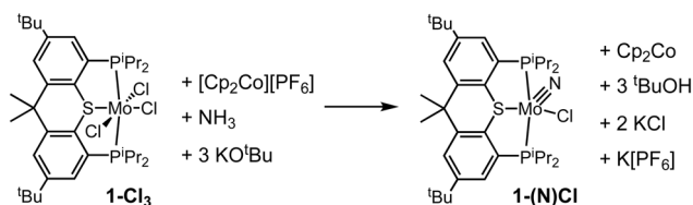
Scheme 8 Ideal balanced equation for reaction (oxidation) of 1-Cl 3 with NH_3 , base, and Cp_2Co^+ . (Actual reaction gives substantial decomposition/ligand-loss).
