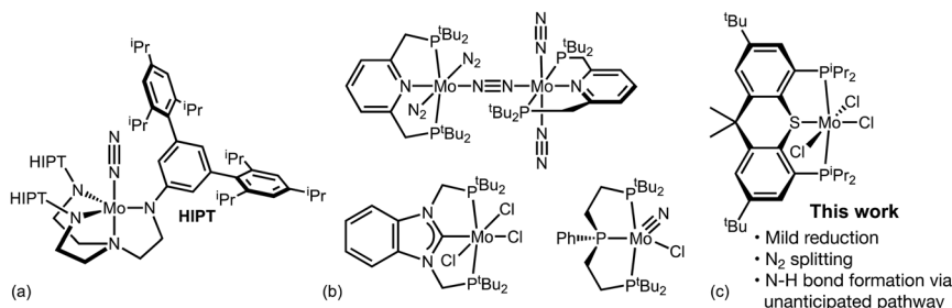
Fig. 1 (a) Schrock's (triamidoamine)Mo catalyst. 19,104 (b) (PNP)Mo catalysts or catalyst precursors reported by Nishibayashi. 20–37 (c) (PSP)Mo complex reported in this work.
