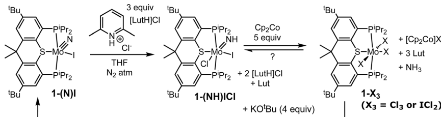
Scheme 7 Reaction of 1-(NH)ICl with [LutH]Cl and Cp_2Co to yield 1-Cl 3 and NH_3 , followed by addition of KOtBu .
