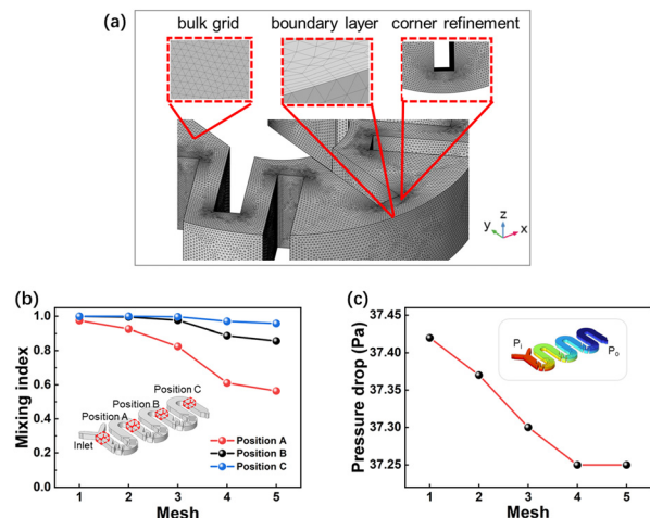
Fig. 3 (a) Schematic diagram of the model grids. (b) The variation of the mixing index at positions A, B, and C of M_3 with the number of grids. (c) The fluctuation of pressure drop at the inlet and outlet of M_3 with the number of grids.
