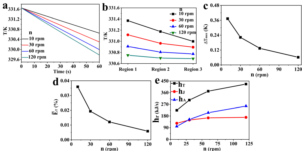
Fig. 8 Effect of agitator speeds on (a) fluid temperature in all reaction zones at different times, (b) average fluid temperature in various regions, (c) \Delta T_{\max} , (d) \bar{E}_T , (e) h_T , h_A , h_J .
