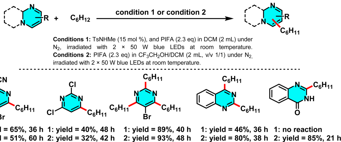
Scheme 80 Metal-free Minisci-type heteroarylation of pyrimidines under visible light using alkanes as radical donors.
