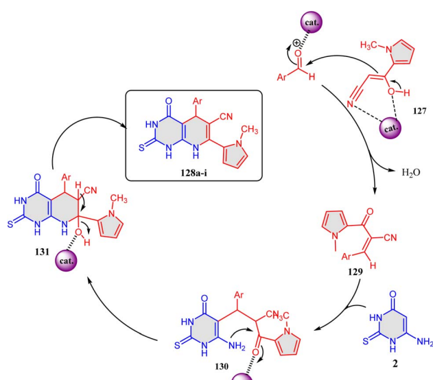
Scheme 44 Suggested mechanism for the synthesis of compound 128 .
