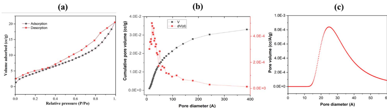
Fig. 4 (a) N_2 adsorption-desorption isotherm of GA@Fe_3O_4 , (b) pore size distribution of GA@Fe_3O_4 determined by the BJH adsorption method, (c) pore size distribution of GA@Fe_3O_4 determined by the DA method.
